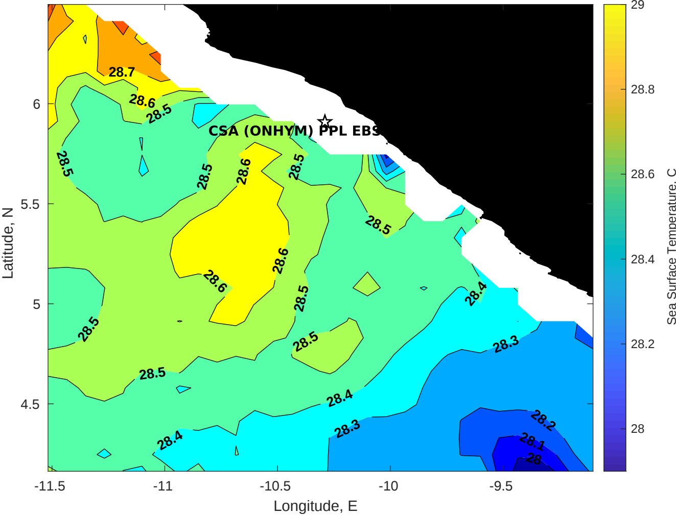
SST for CSA (ONHYM) PPL EBS - Liberia at 30-Nov-2025 00:00:00
