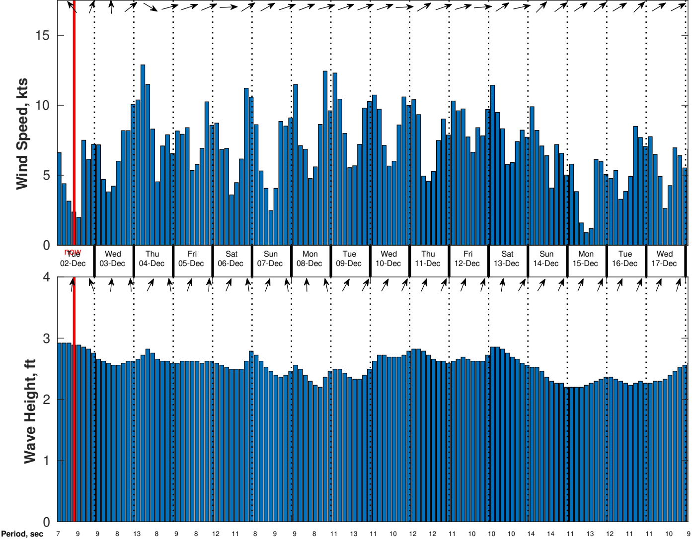
Wind & Wave Forecast for CSA (ONHYM) PPL EBS - Liberia from 01-Dec-2025 01:00:00 to 17-Dec-2025 01:00:00
