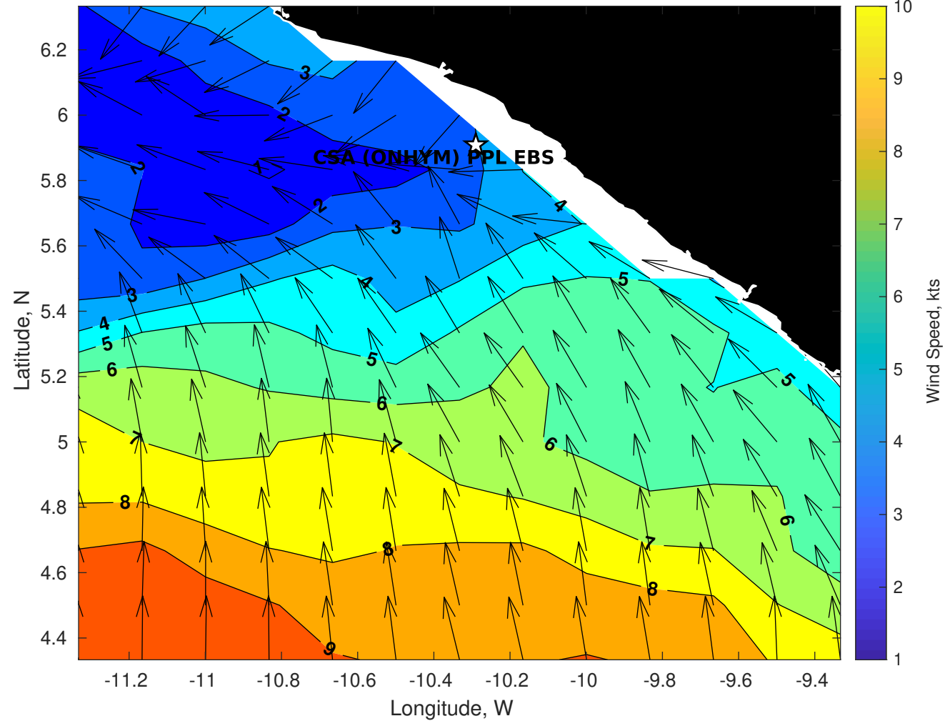
GFS Winds (kts) for CSA (ONHYM) PPL EBS - Liberia at 01-Dec-2025 09:00:00
