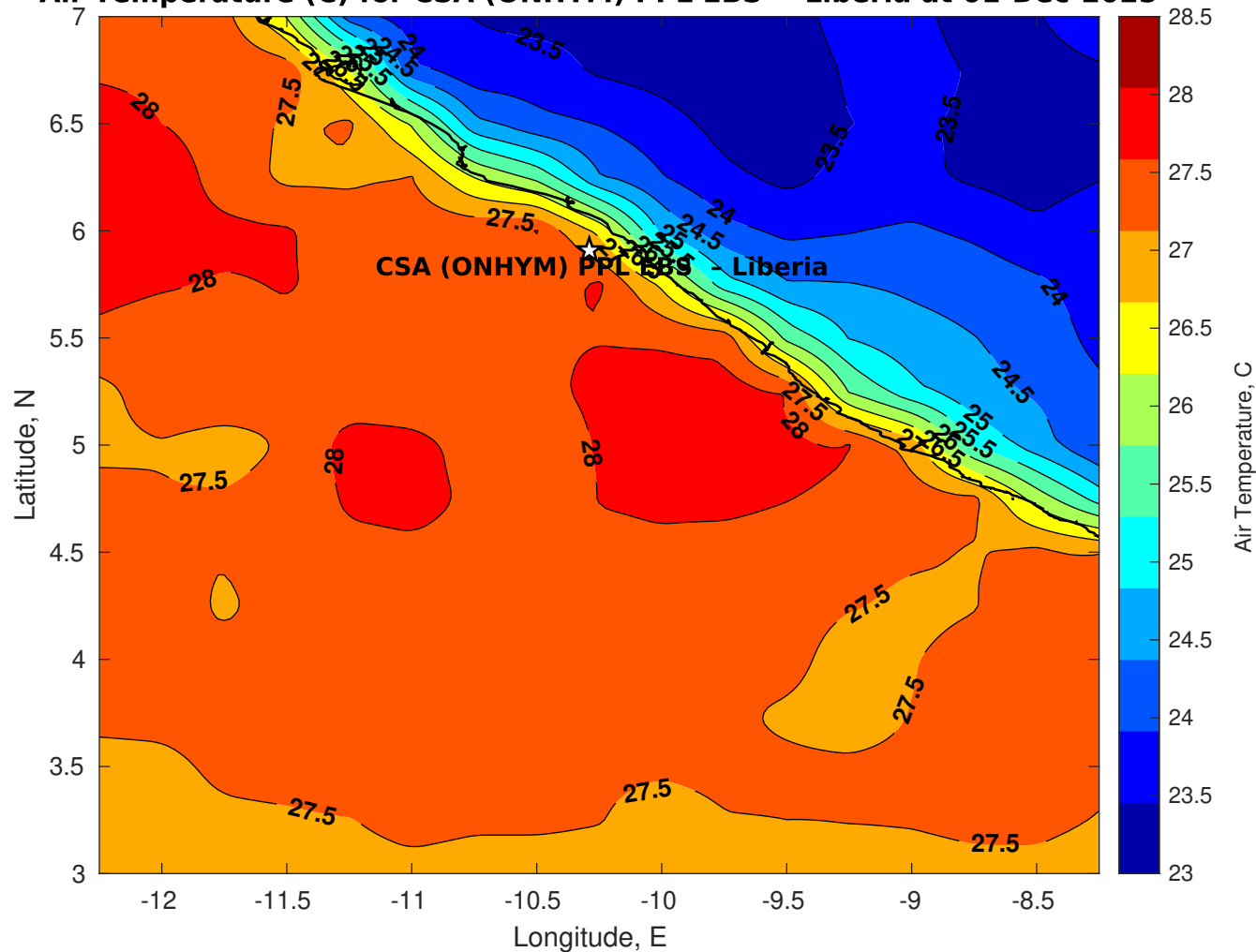
Air Temperature (C) for CSA (ONHYM) PPL EBS - Liberia at 01-Dec-2025
