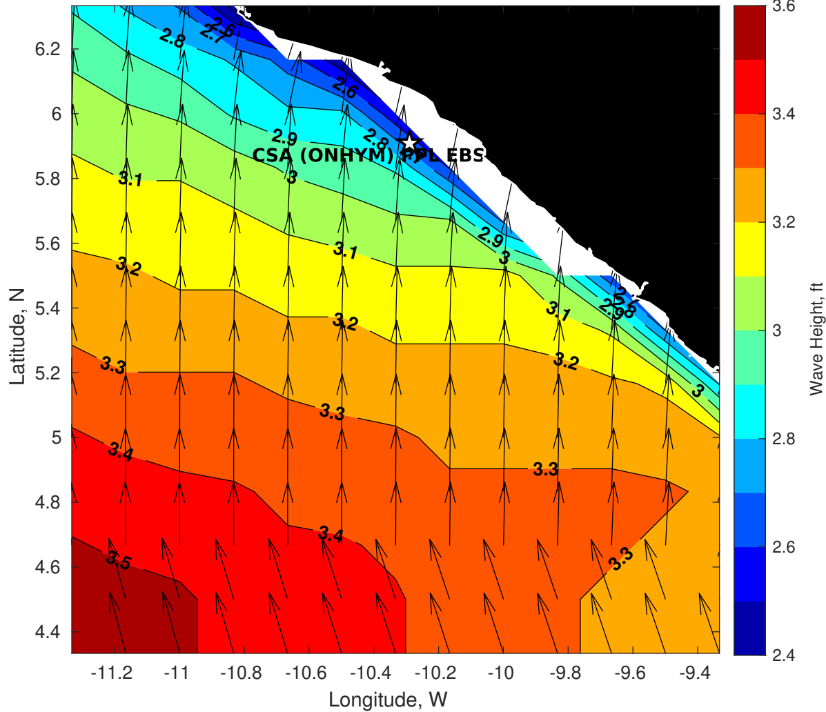
GFS Wave Height (ft) for CSA (ONHYM) PPL EBS - Liberia at 01-Dec-2025 09:00:00
