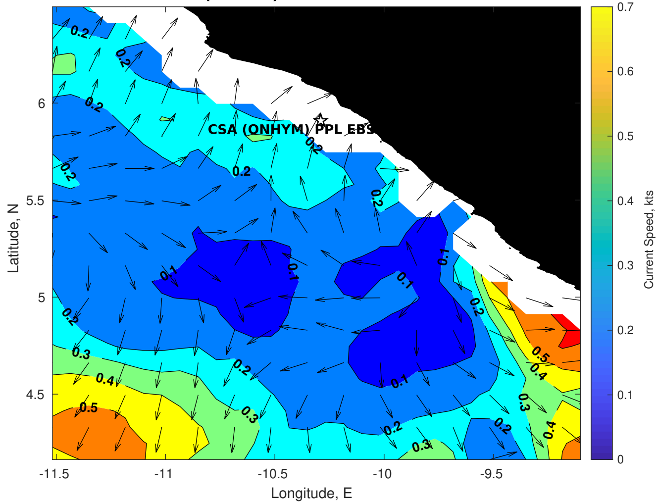
Surface Currents for CSA (ONHYM) PPL EBS - Liberia at 30-Nov-2025 00:00:00
