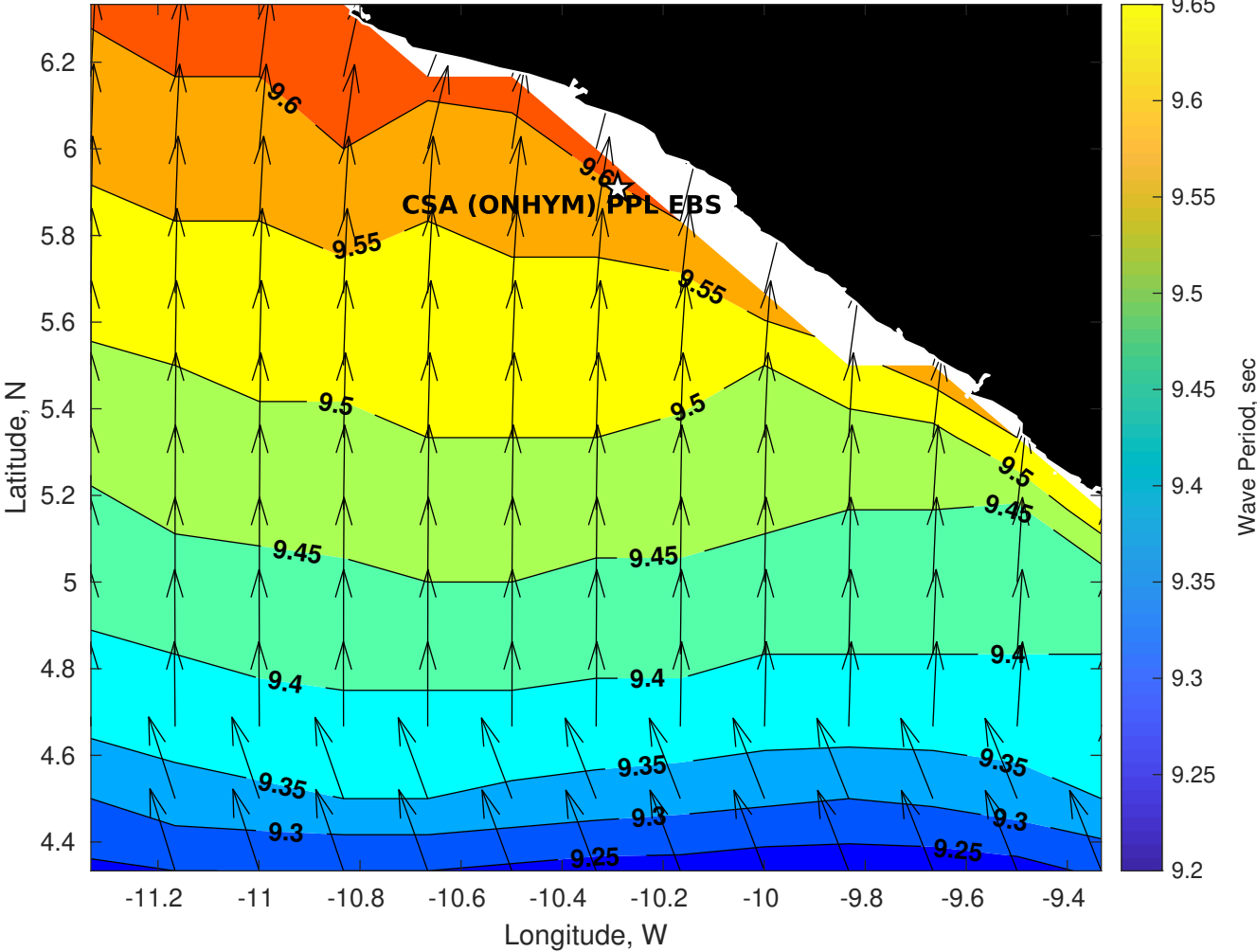
GFS Wave Period (sec) for CSA (ONHYM) PPL EBS - Liberia at 01-Dec-2025 09:00:00
