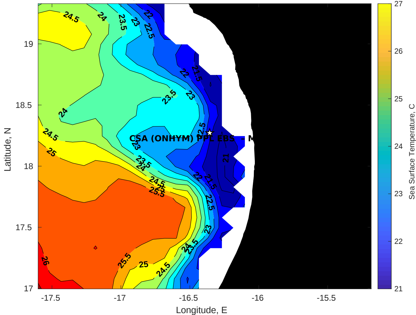
SST for CSA (ONHYM) PPL EBS - Mauritania at 30-Nov-2025 00:00:00
