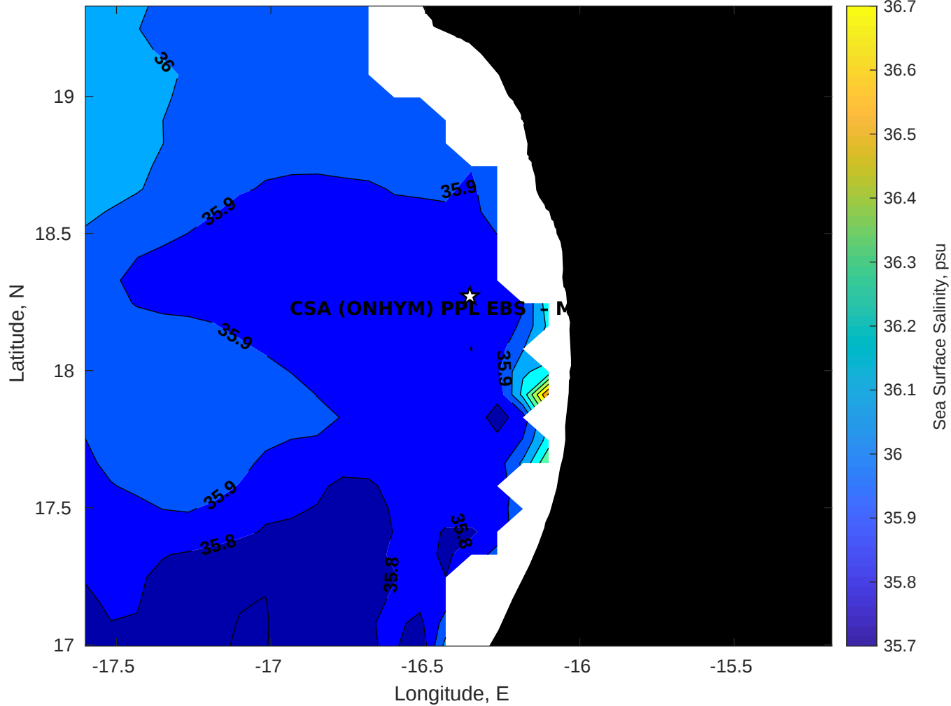
Surface Salinity for CSA (ONHYM) PPL EBS - Mauritania at 30-Nov-2025 00:00:00
