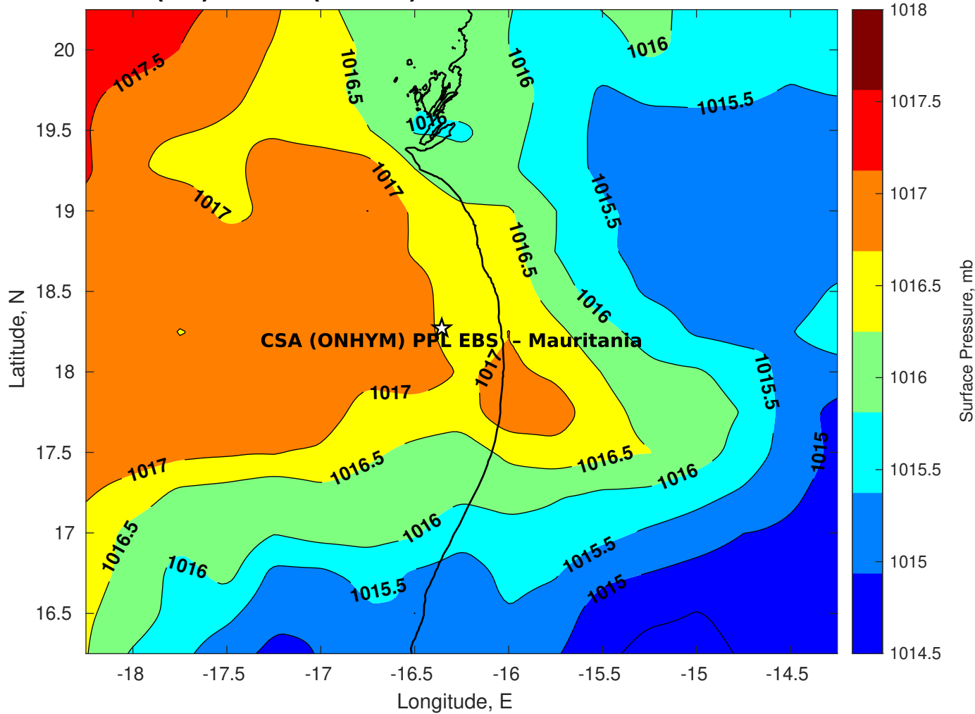
Surface Pressure (mb) for CSA (ONHYM) PPL EBS - Mauritania at 03-Dec-2025 00:00:00
