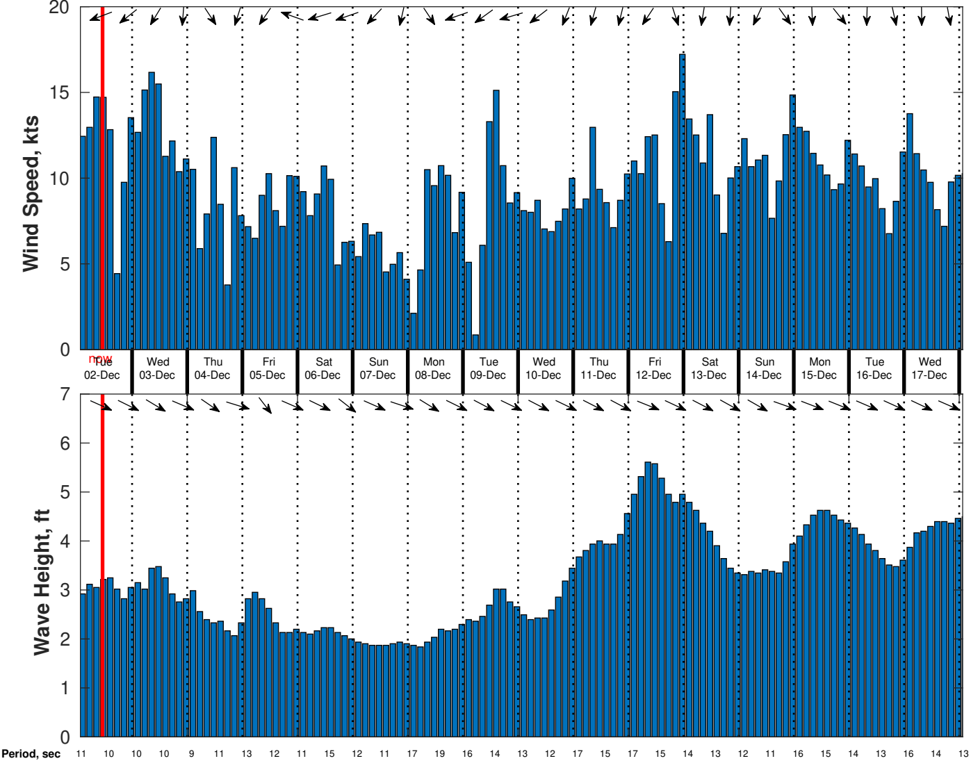
Wind & Wave Forecast for CSA (ONHYM) PPL EBS - Mauritania from 01-Dec-2025 01:00:00 to 17-Dec-2025 01:00:00
