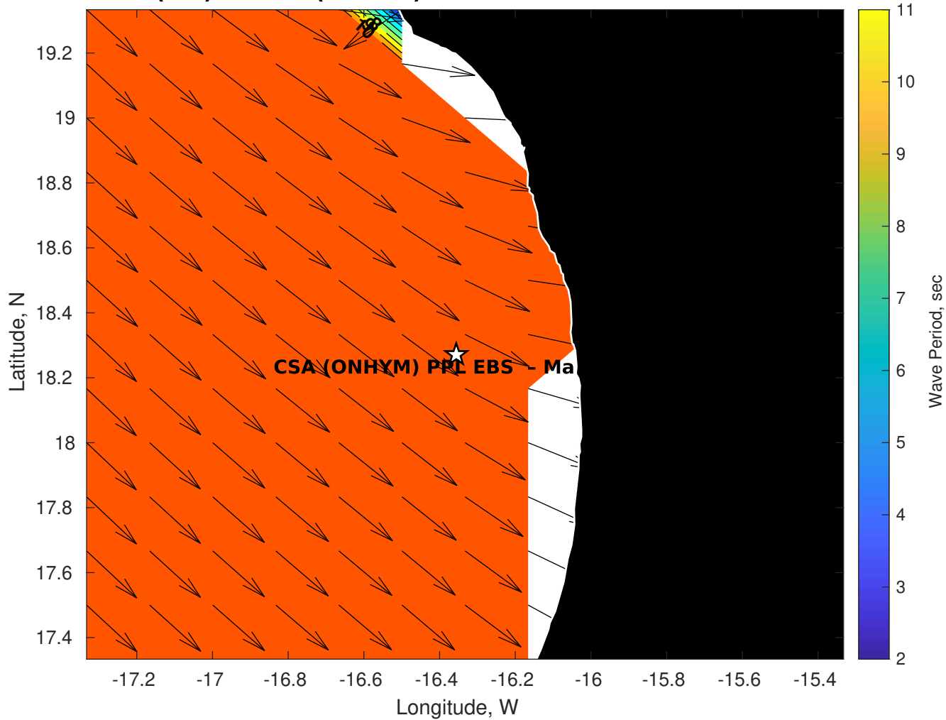
GFS Wave Period (sec) for CSA (ONHYM) PPL EBS - Mauritania at 01-Dec-2025 09:00:00
