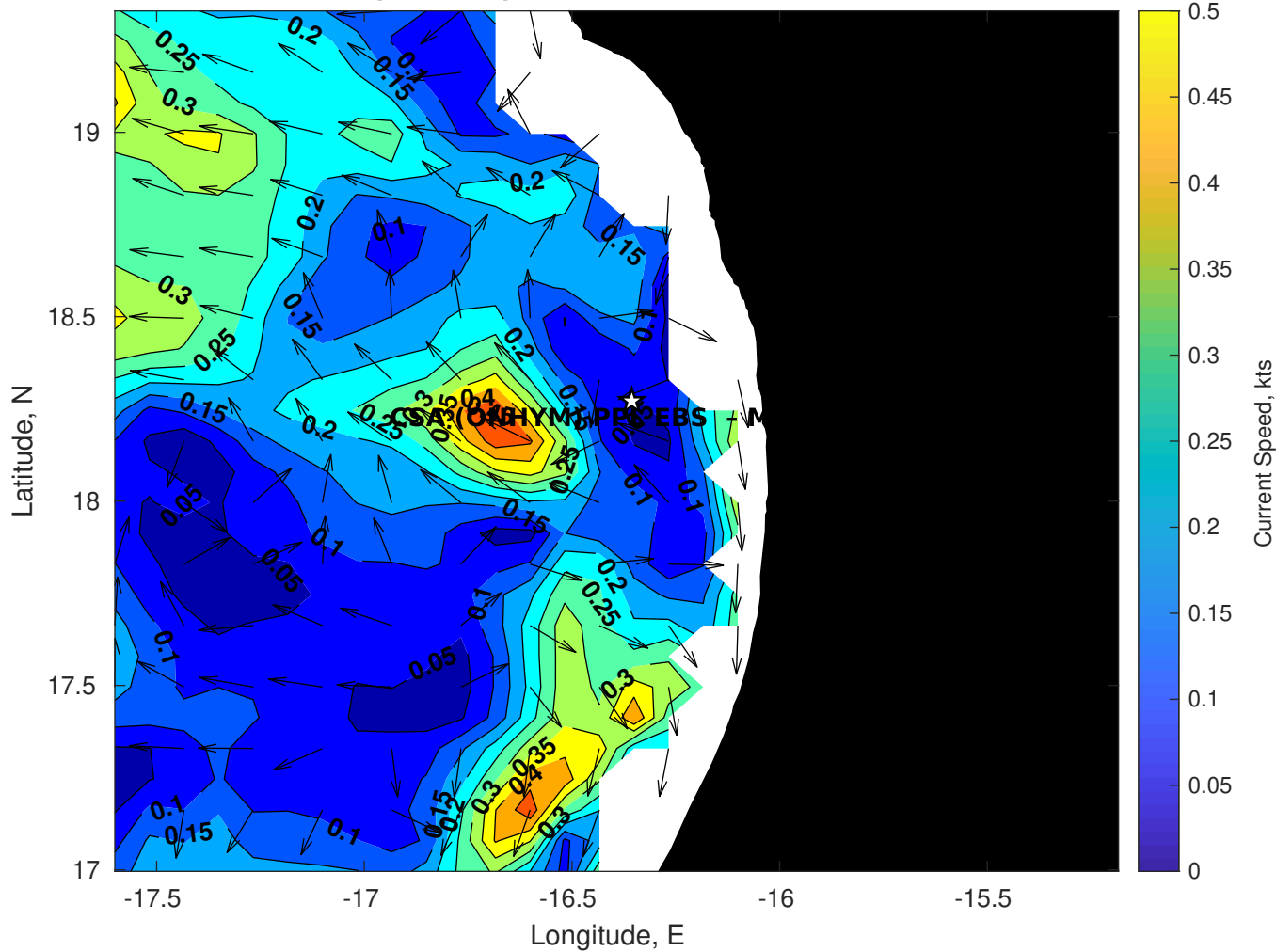
Surface Currents for CSA (ONHYM) PPL EBS - Mauritania at 30-Nov-2025 00:00:00
