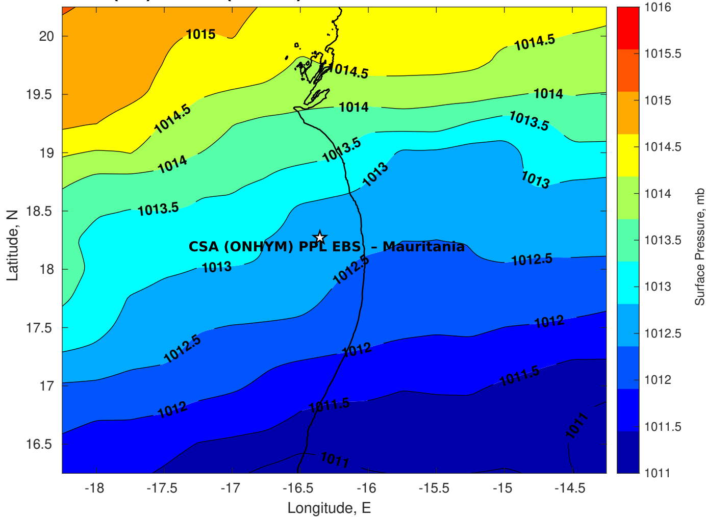
Surface Pressure (mb) for CSA (ONHYM) PPL EBS - Mauritania at 02-Dec-2025 00:00:00
