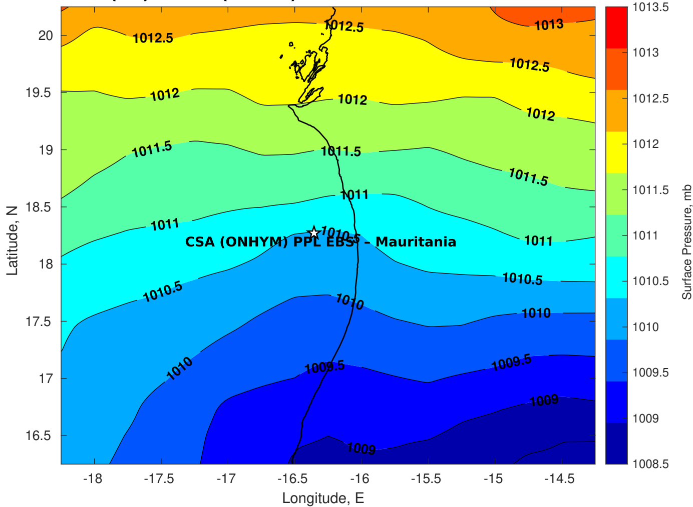
Surface Pressure (mb) for CSA (ONHYM) PPL EBS - Mauritania at 01-Dec-2025 00:00:00
