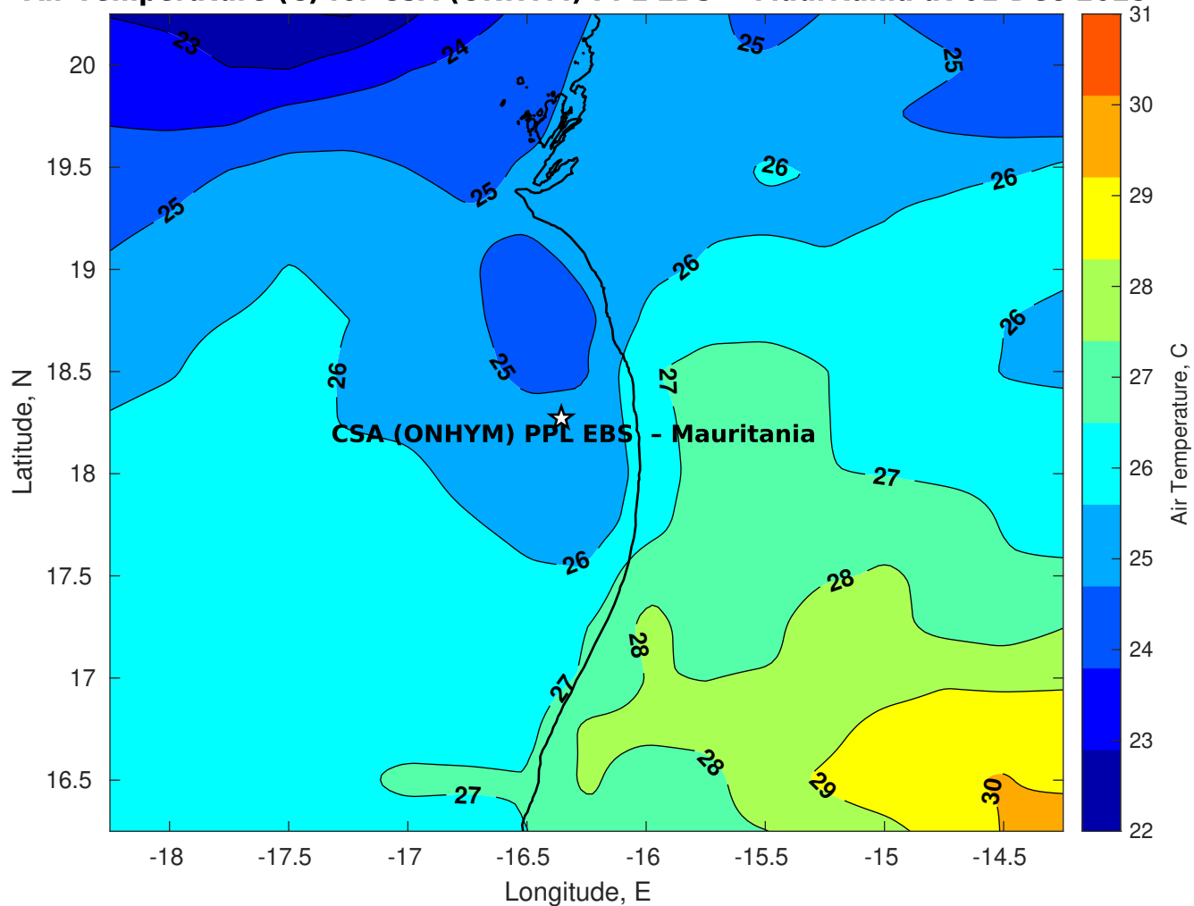
Air Temperature (C) for CSA (ONHYM) PPL EBS - Mauritania at 01-Dec-2025
