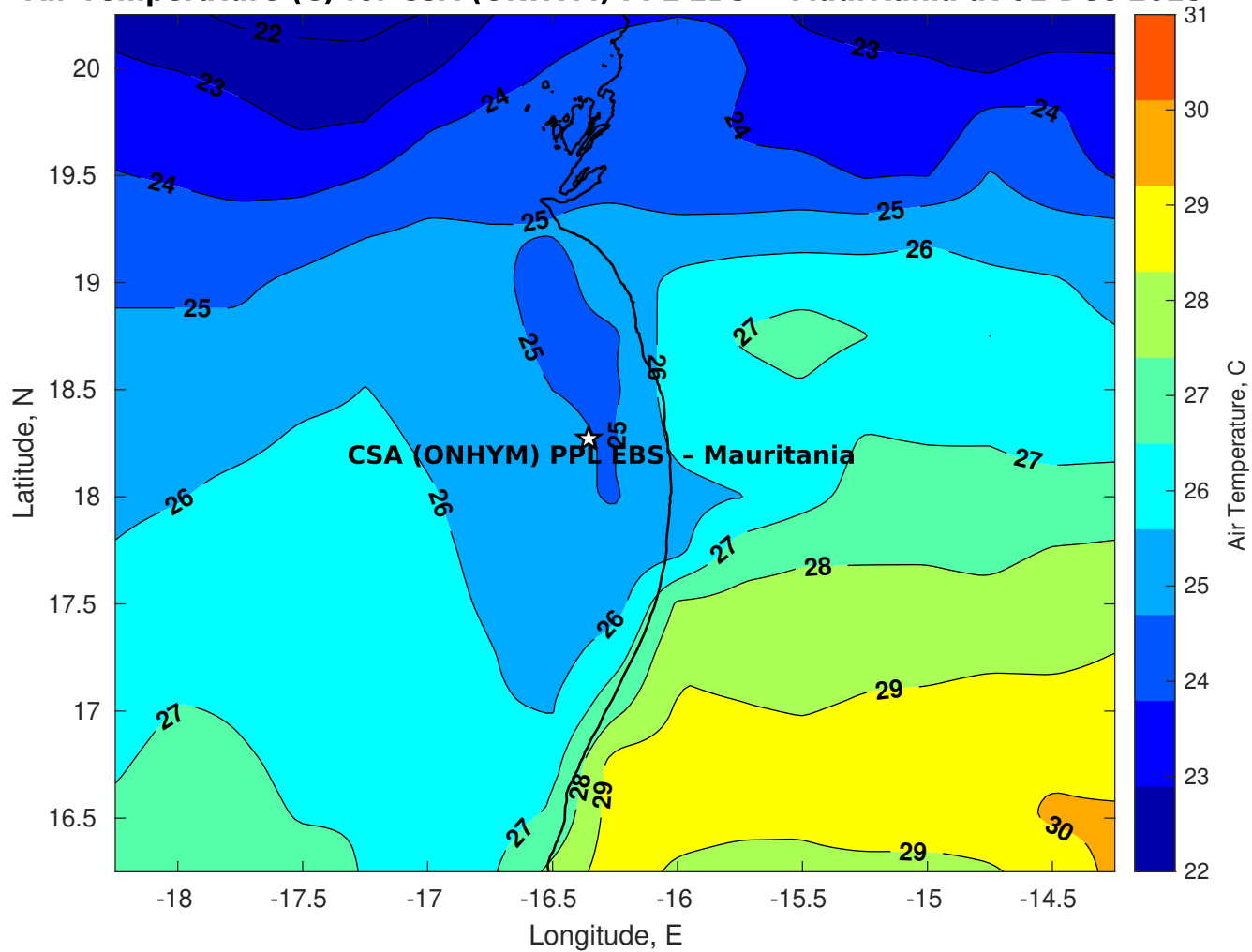
Air Temperature (C) for CSA (ONHYM) PPL EBS - Mauritania at 01-Dec-2025
