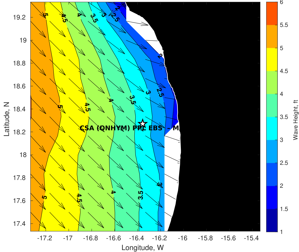
GFS Wave Height (ft) for CSA (ONHYM) PPL EBS - Mauritania at 01-Dec-2025 09:00:00
