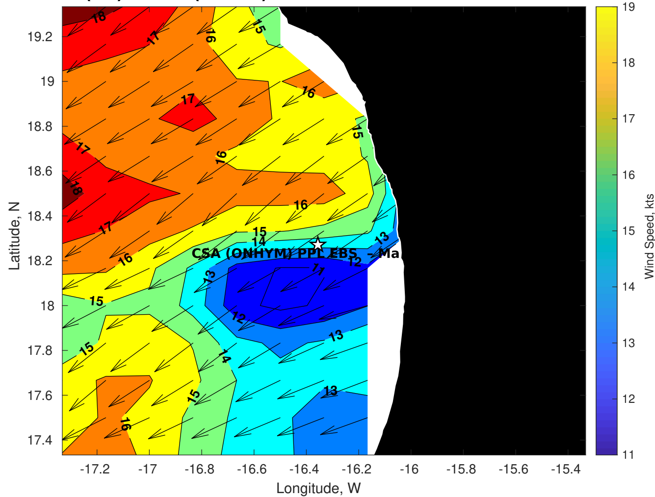
GFS Winds (kts) for CSA (ONHYM) PPL EBS - Mauritania at 01-Dec-2025 09:00:00
