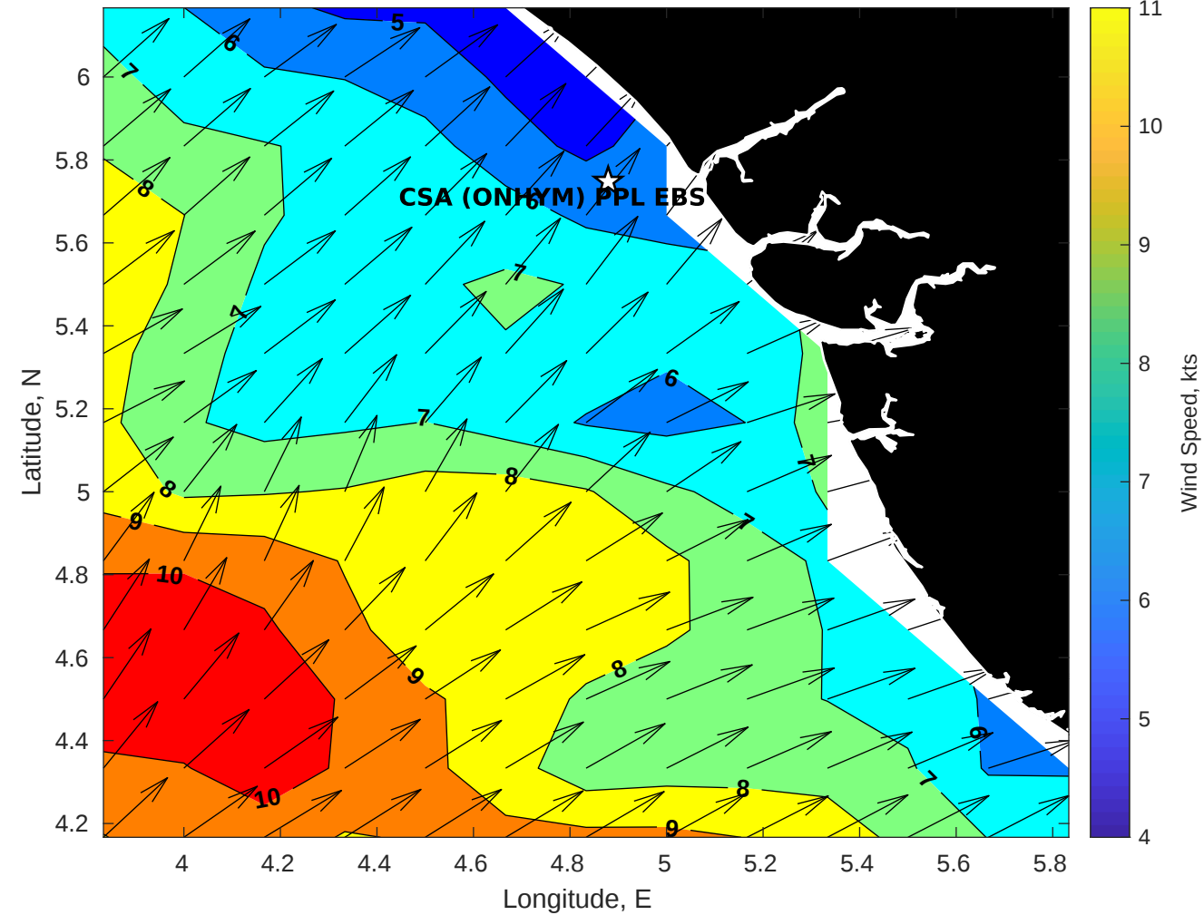
GFS Winds (kts) for CSA (ONHYM) PPL EBS - Nigeria at 01-Dec-2025 09:00:00
