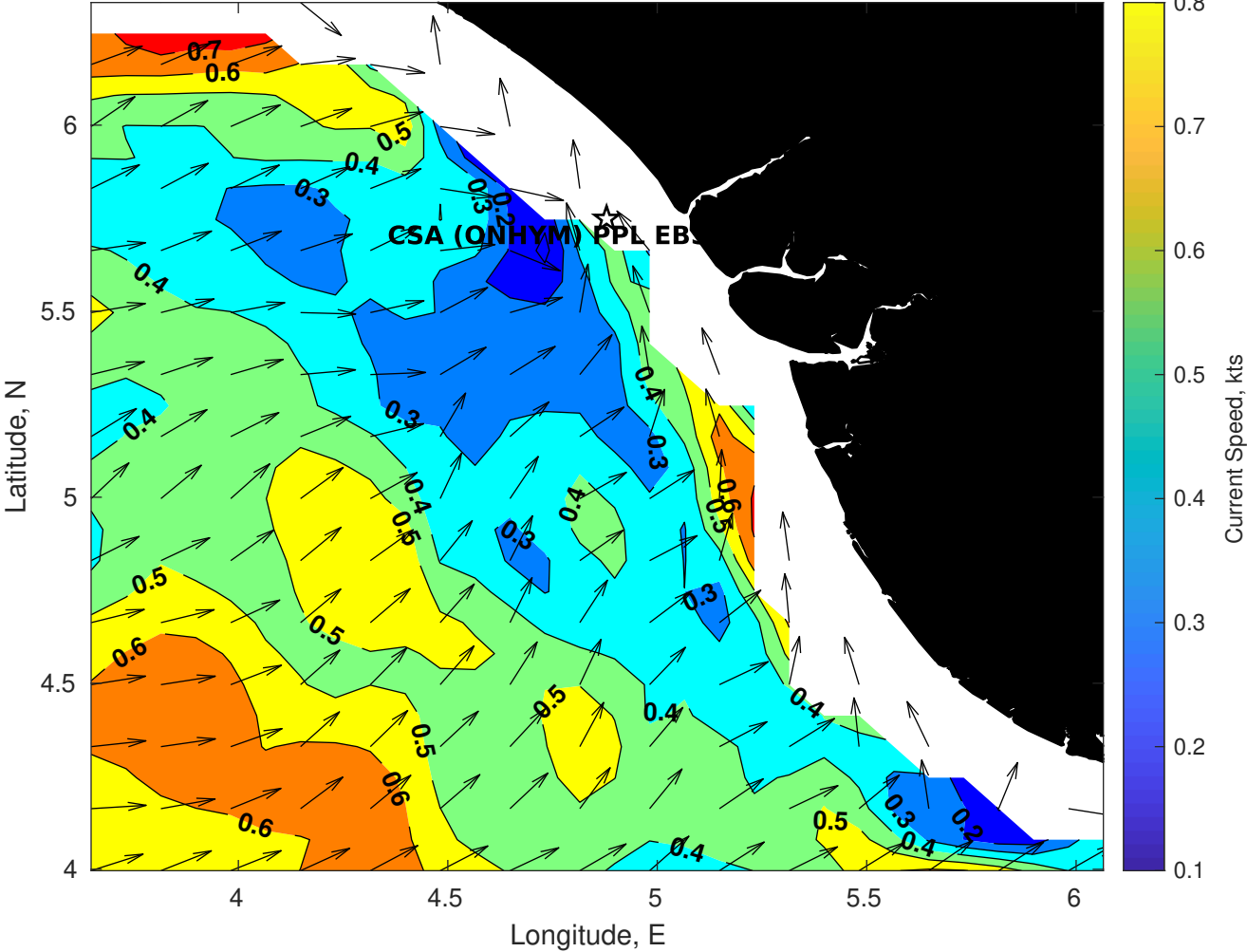
Surface Currents for CSA (ONHYM) PPL EBS - Nigeria at 30-Nov-2025 00:00:00
