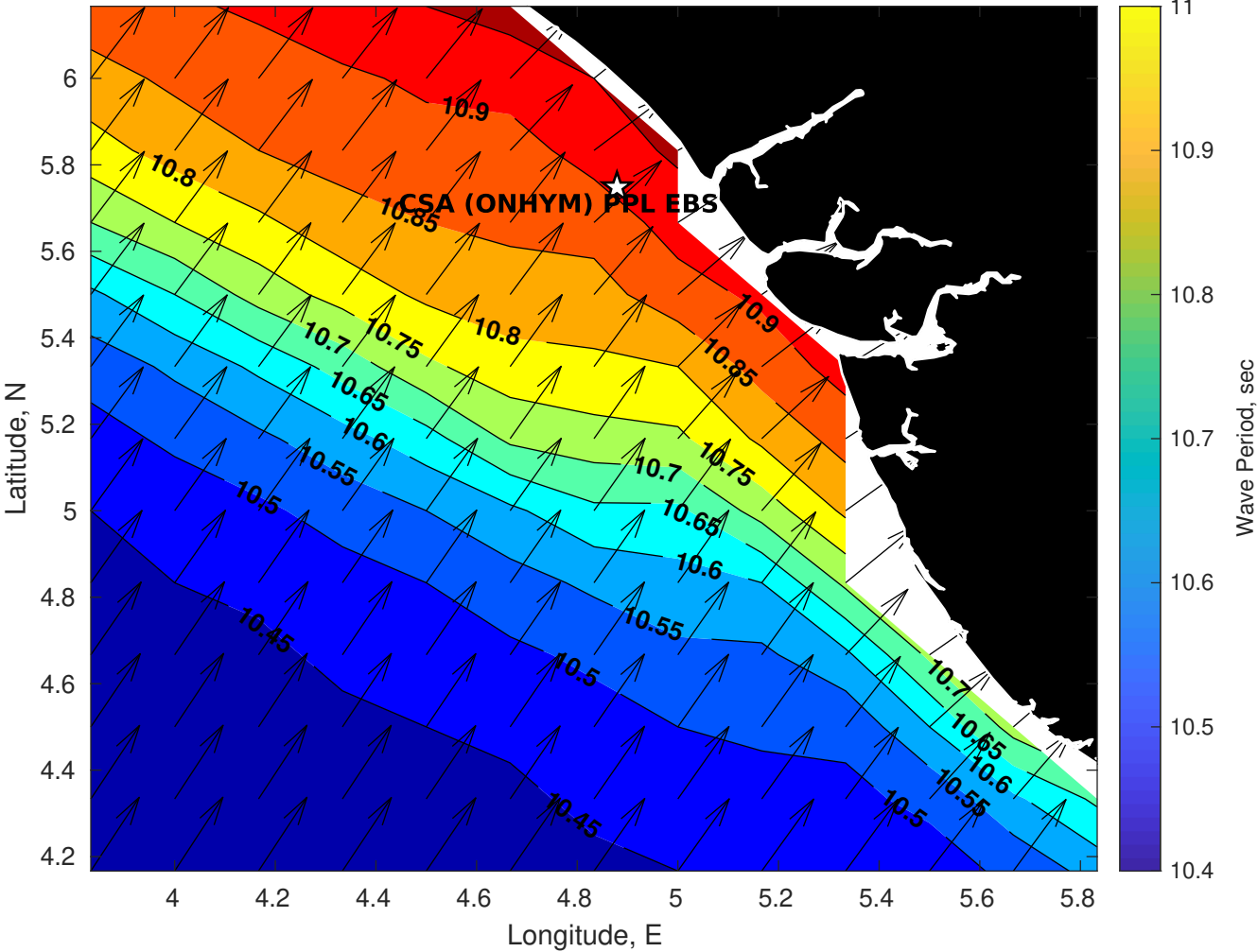
GFS Wave Period (sec) for CSA (ONHYM) PPL EBS - Nigeria at 01-Dec-2025 09:00:00
