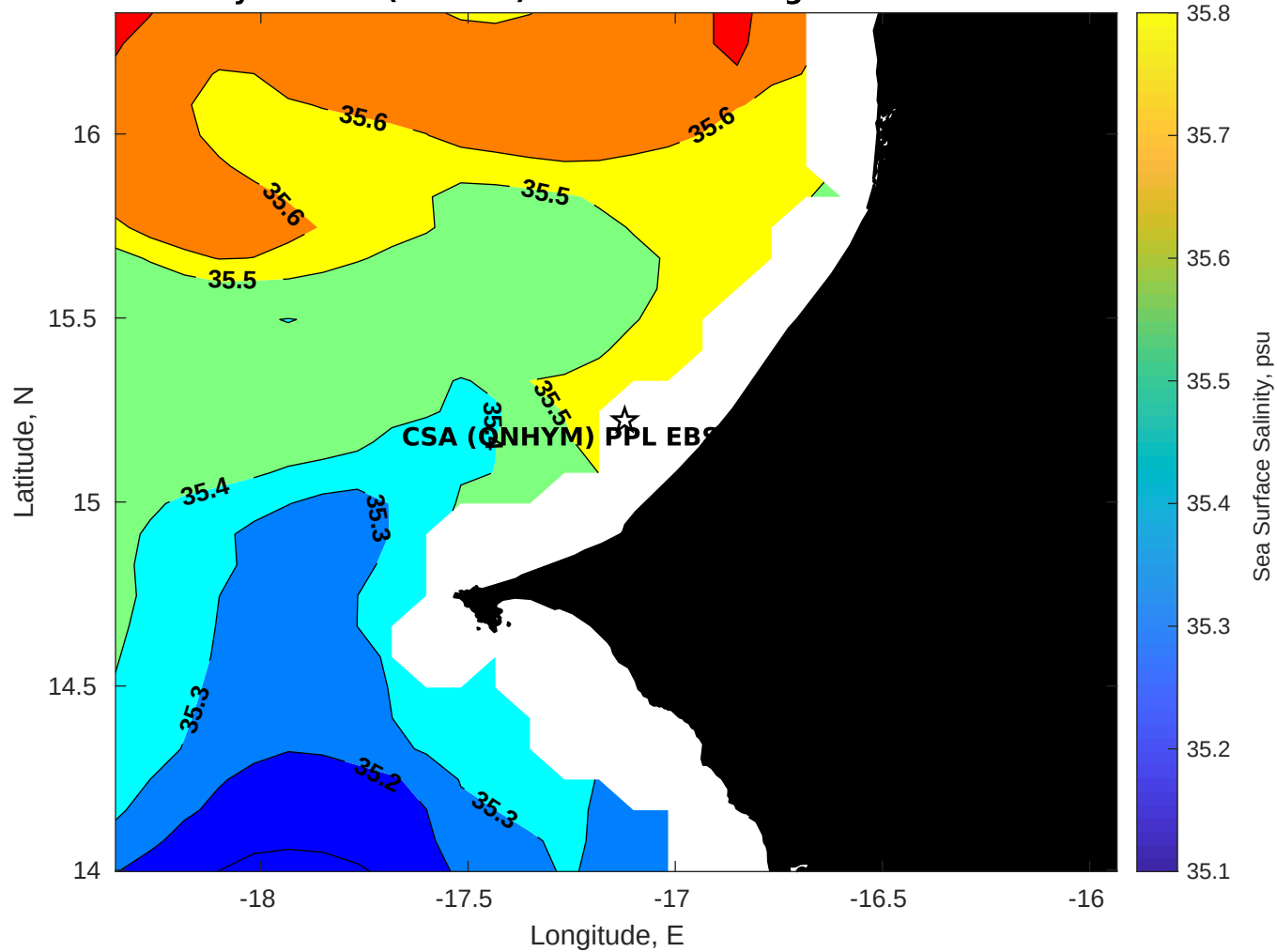
Surface Salinity for CSA (ONHYM) PPL EBS - Senegal at 30-Nov-2025 00:00:00
