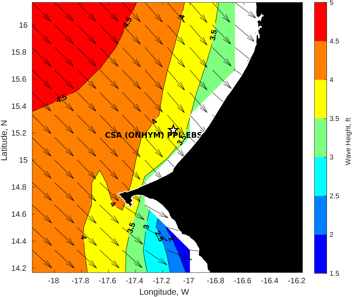
GFS Wave Height (ft) for CSA (ONHYM) PPL EBS - Senegal at 01-Dec-2025 09:00:00
