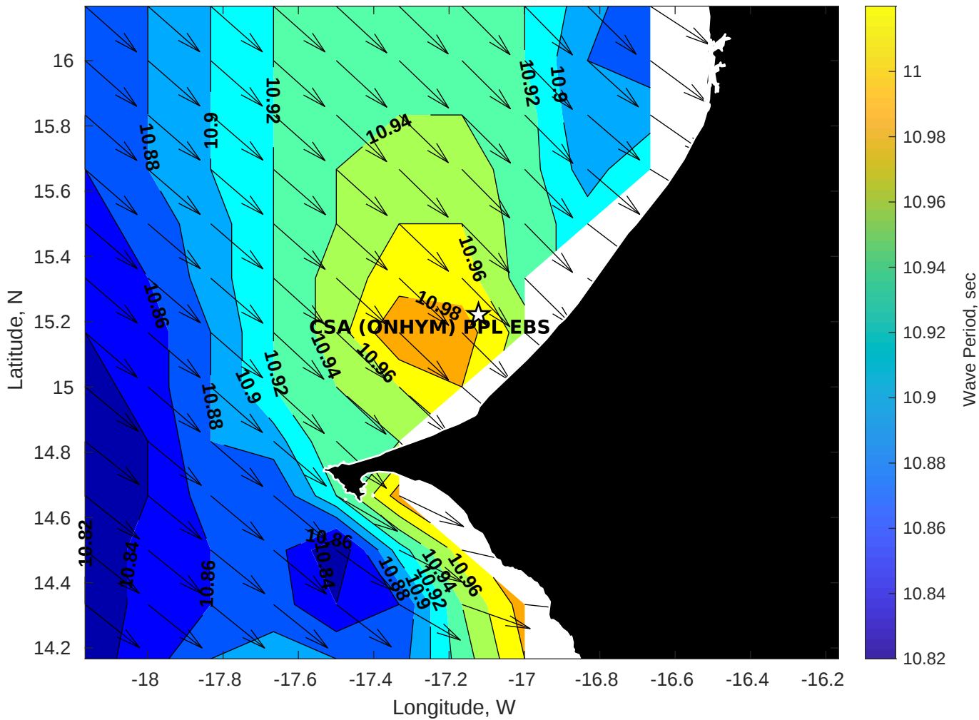
GFS Wave Period (sec) for CSA (ONHYM) PPL EBS - Senegal at 01-Dec-2025 09:00:00
