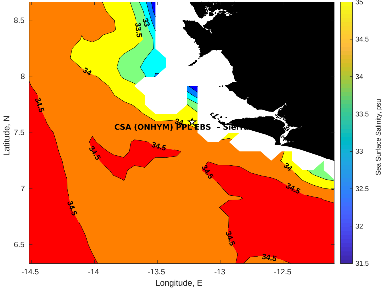
Surface Salinity for CSA (ONHYM) PPL EBS - Sierra Leone at 30-Nov-2025 00:00:00
