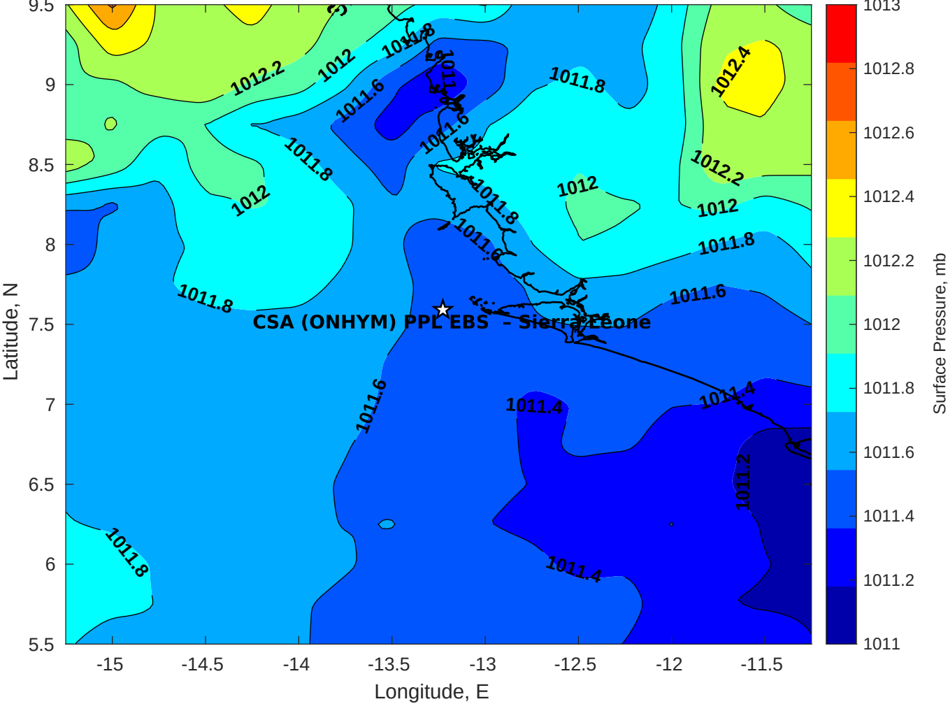
Surface Pressure (mb) for CSA (ONHYM) PPL EBS - Sierra Leone at 03-Dec-2025 00:00:00
