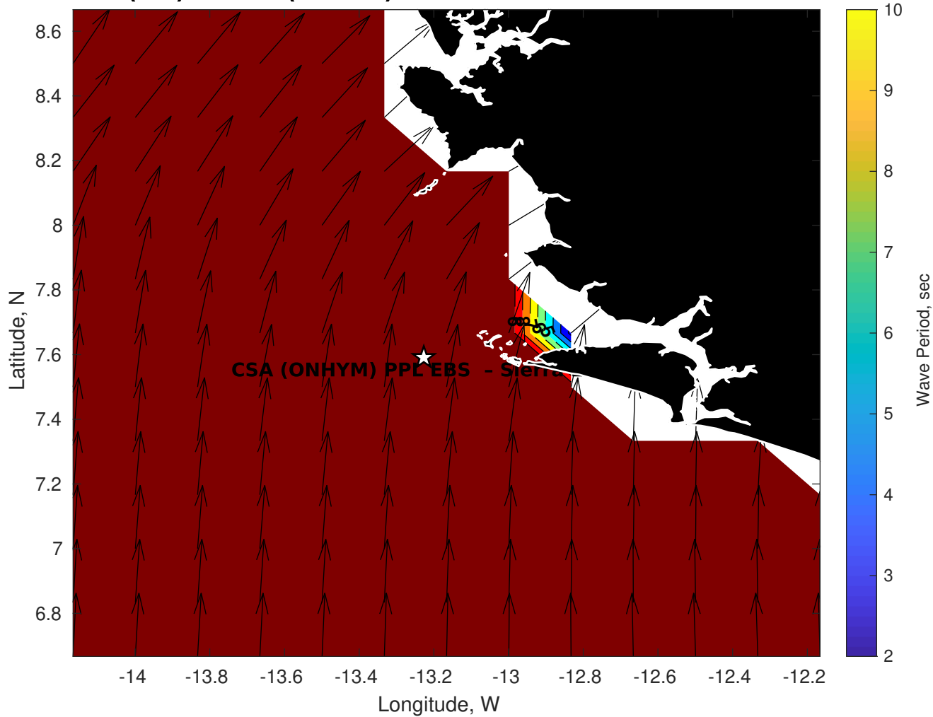
GFS Wave Period (sec) for CSA (ONHYM) PPL EBS - Sierra Leone at 01-Dec-2025 09:00:00
