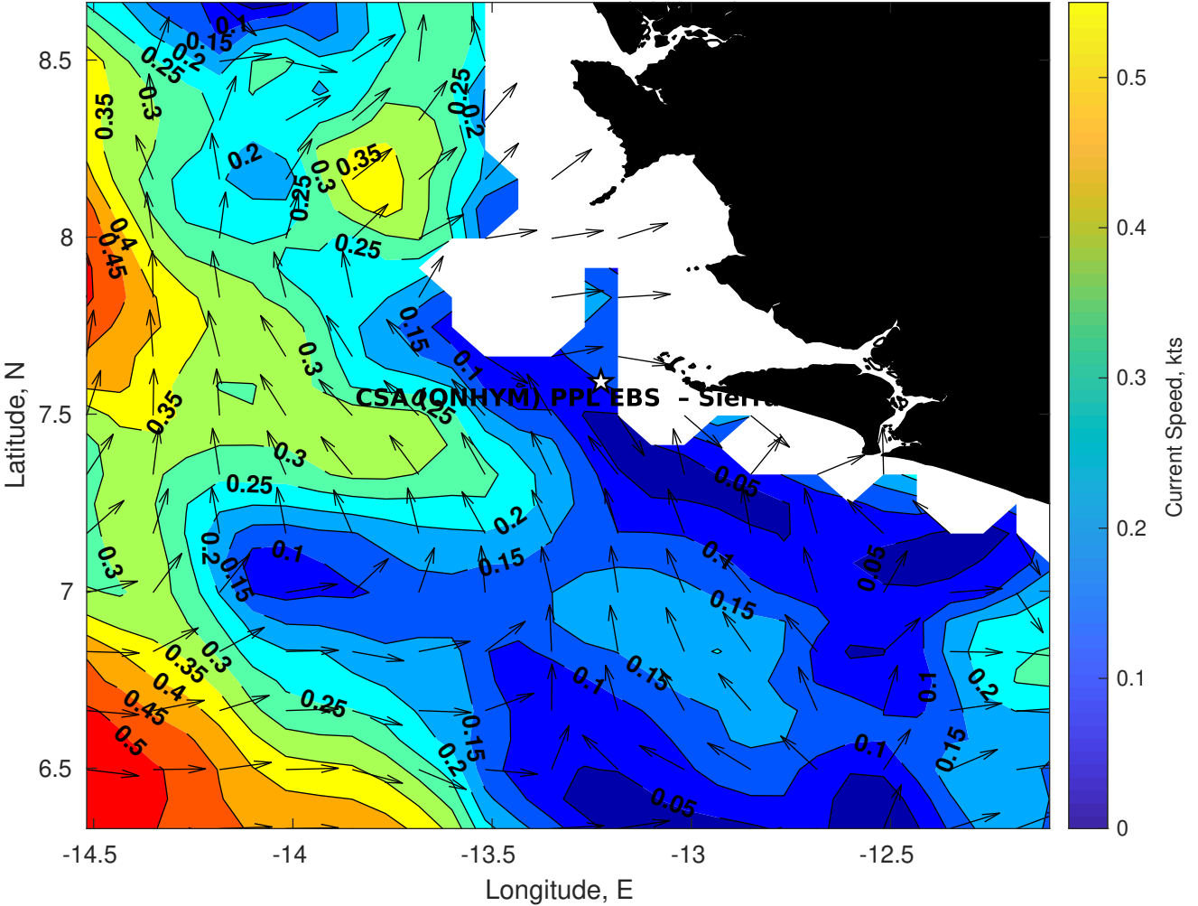
Surface Currents for CSA (ONHYM) PPL EBS - Sierra Leone at 30-Nov-2025 00:00:00
