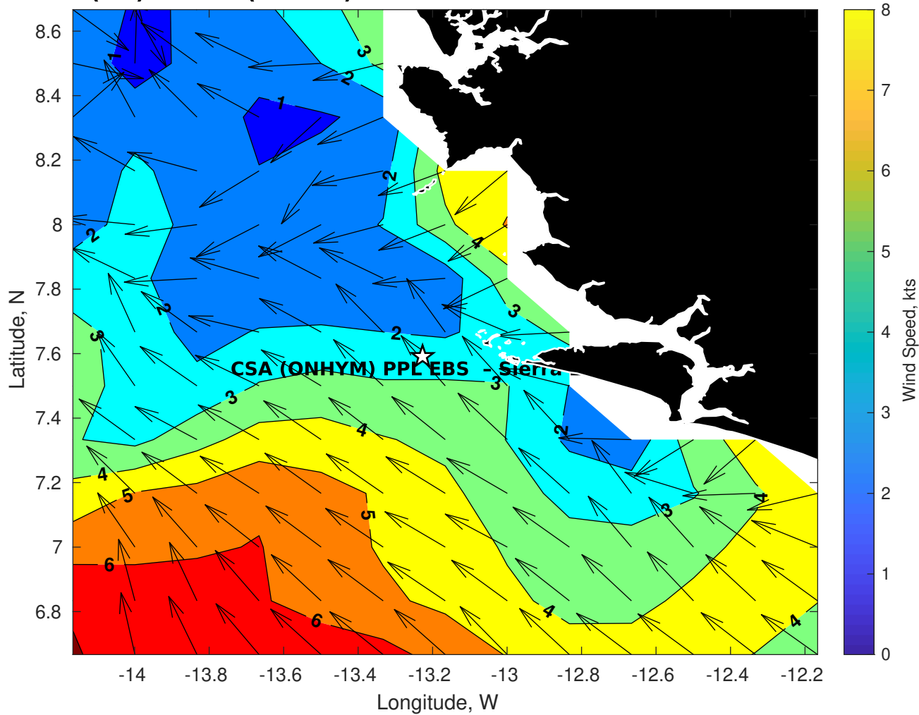
GFS Winds (kts) for CSA (ONHYM) PPL EBS - Sierra Leone at 01-Dec-2025 09:00:00
