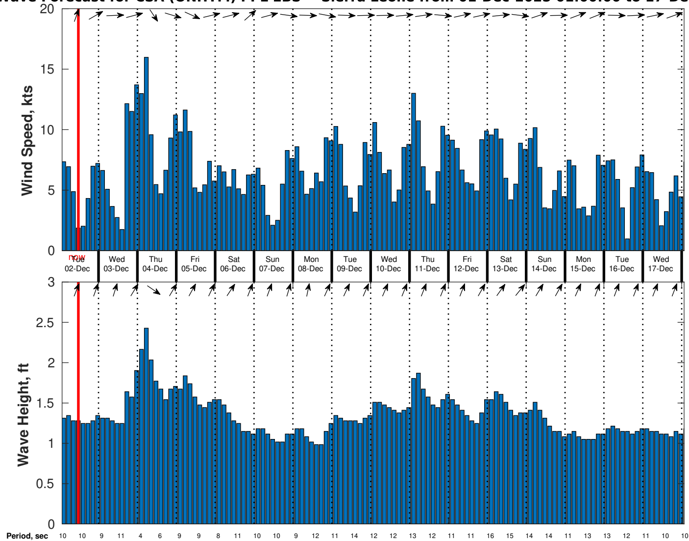
Wind & Wave Forecast for CSA (ONHYM) PPL EBS - Sierra Leone from 01-Dec-2025 01:00:00 to 17-Dec-2025 01:00:00
