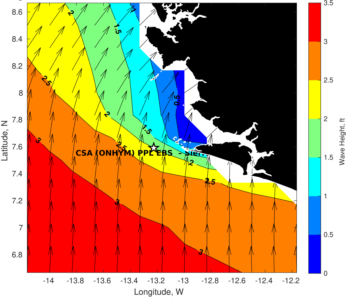
GFS Wave Height (ft) for CSA (ONHYM) PPL EBS - Sierra Leone at 01-Dec-2025 09:00:00
