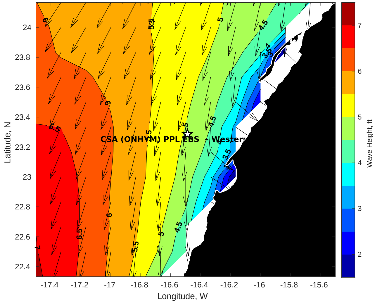
GFS Wave Height (ft) for CSA (ONHYM) PPL EBS - Western Sahara at 01-Dec-2025 09:00:00
