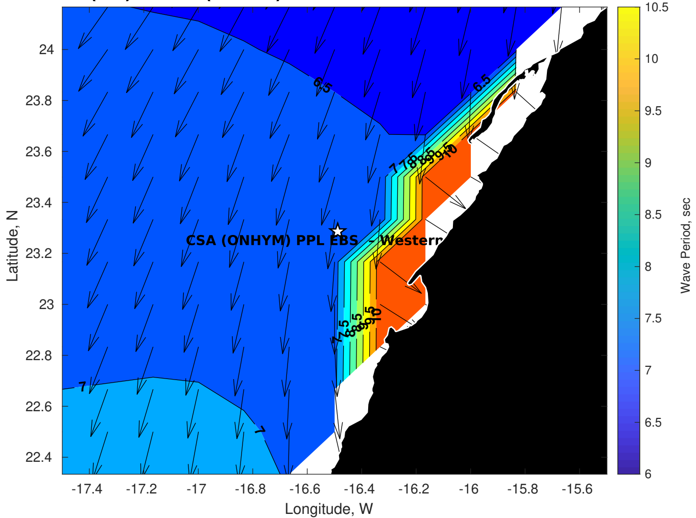
GFS Wave Period (sec) for CSA (ONHYM) PPL EBS - Western Sahara at 01-Dec-2025 09:00:00
