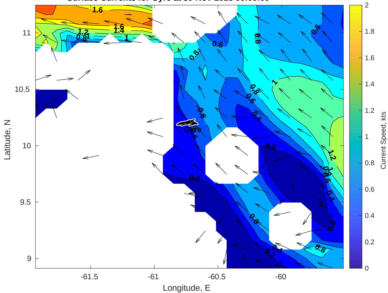
Surface Currents for Gyre at 30-Nov-2025 00:00:00
