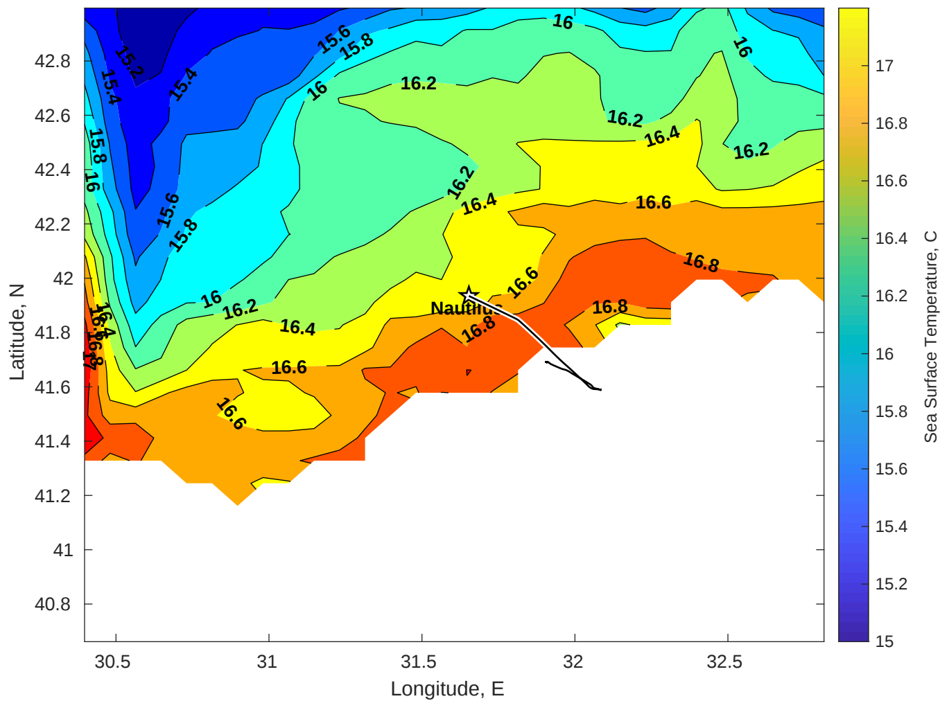
SST for Nautilus at 30-Nov-2025 00:00:00
