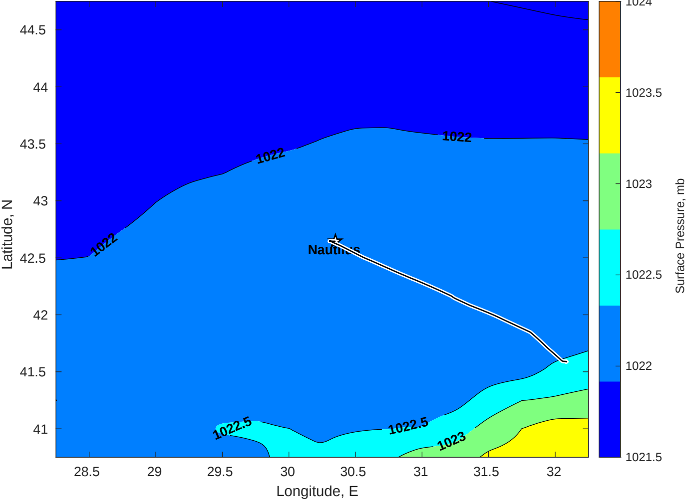
Surface Pressure (mb) for Nautilus at 02-Dec-2025 00:00:00
