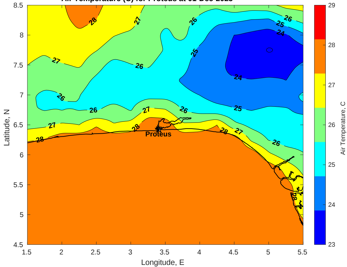
Air Temperature (C) for Proteus at 01-Dec-2025
