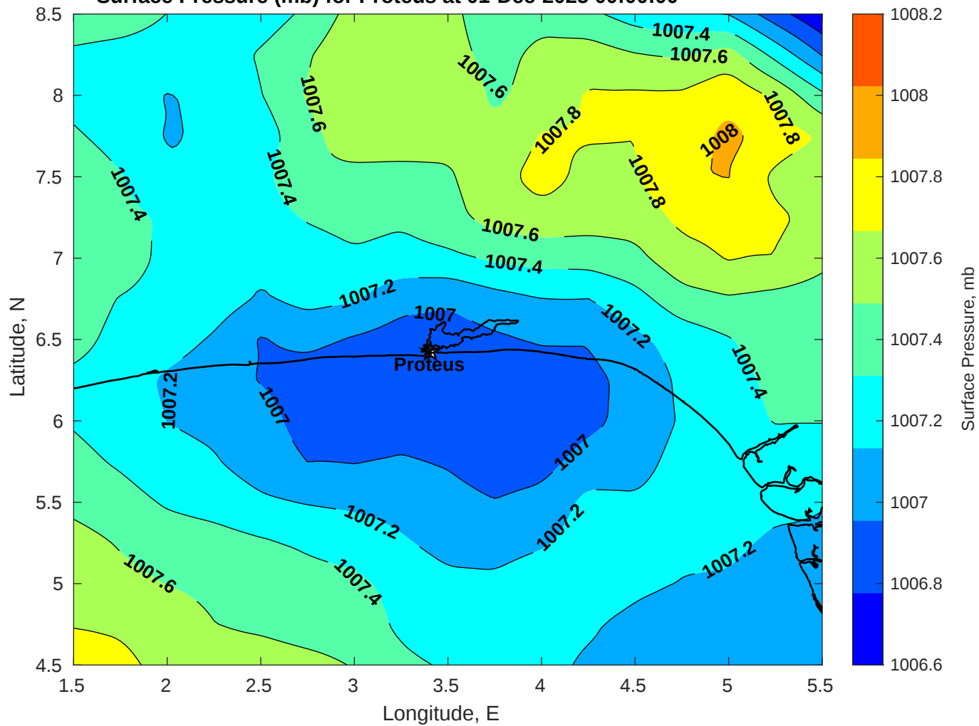
Surface Pressure (mb) for Proteus at 01-Dec-2025 00:00:00
