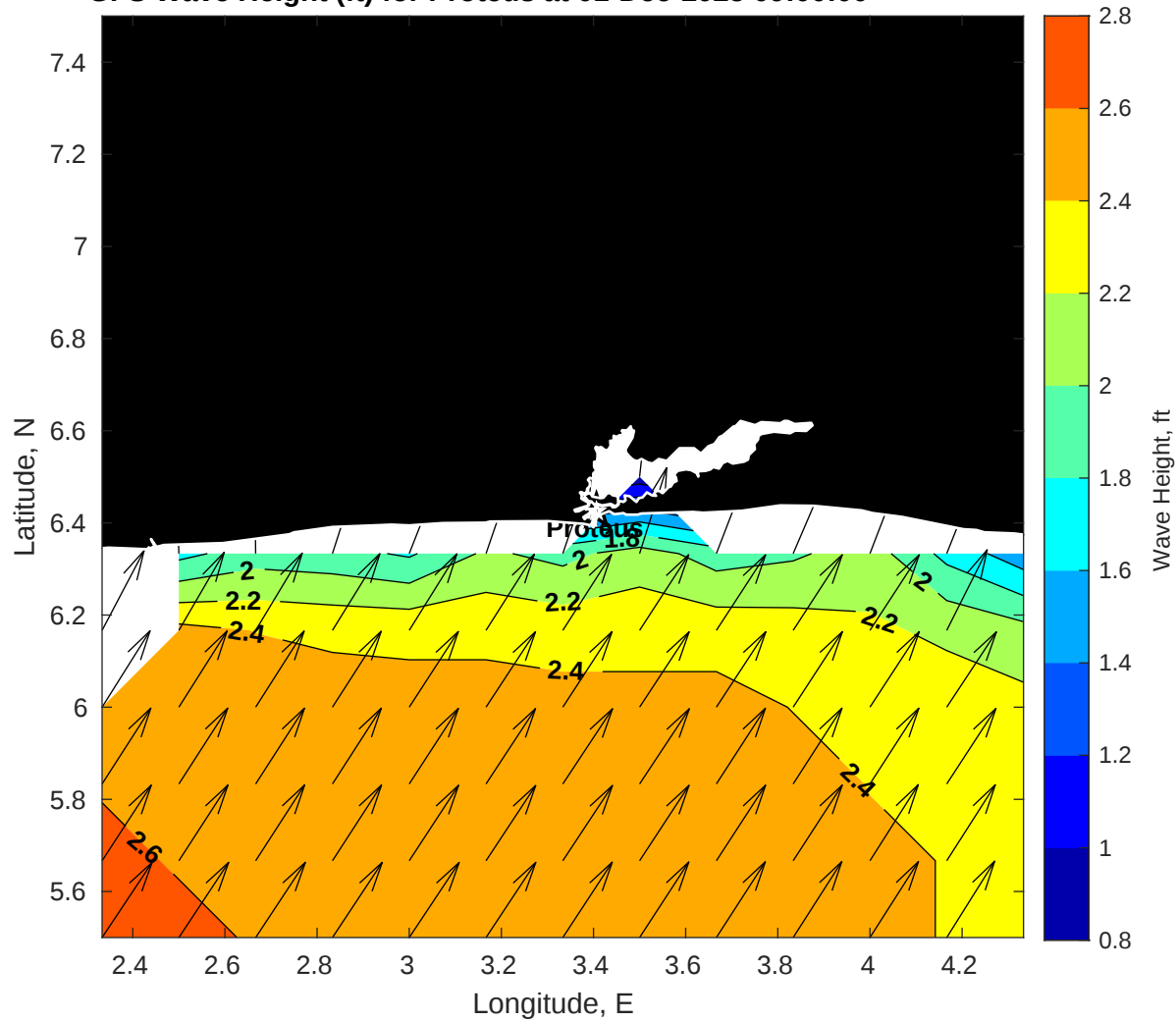
GFS Wave Height (ft) for Proteus at 01-Dec-2025 09:00:00
