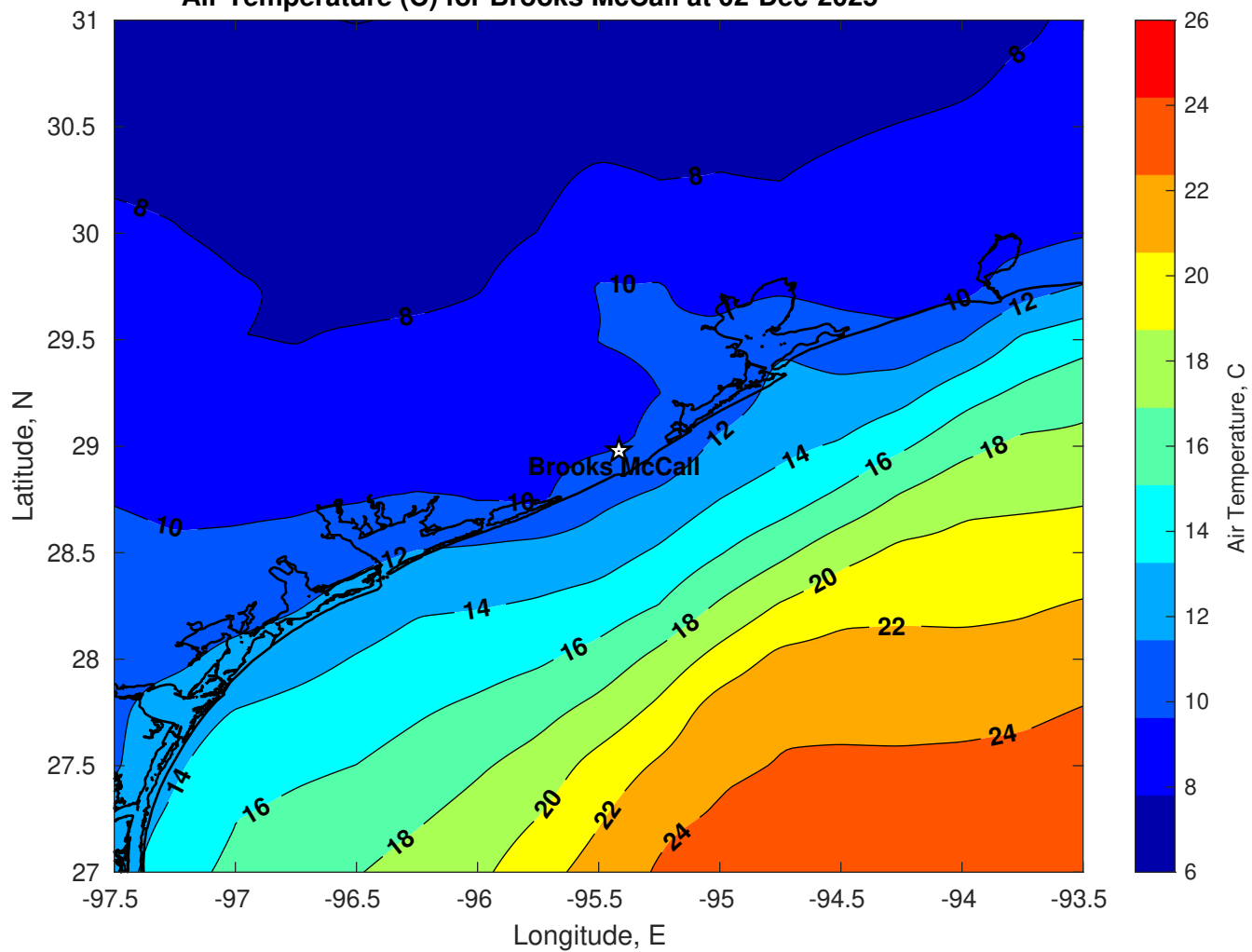
Air Temperature (C) for Brooks McCall at 02-Dec-2025
