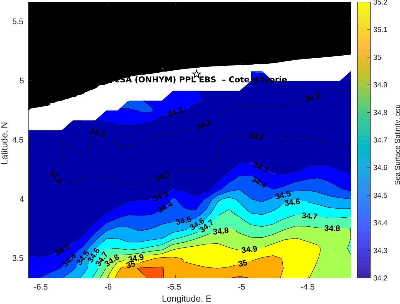
Surface Salinity for CSA (ONHYM) PPL EBS - Cote d'Ivoire at 01-Dec-2025 00:00:00
