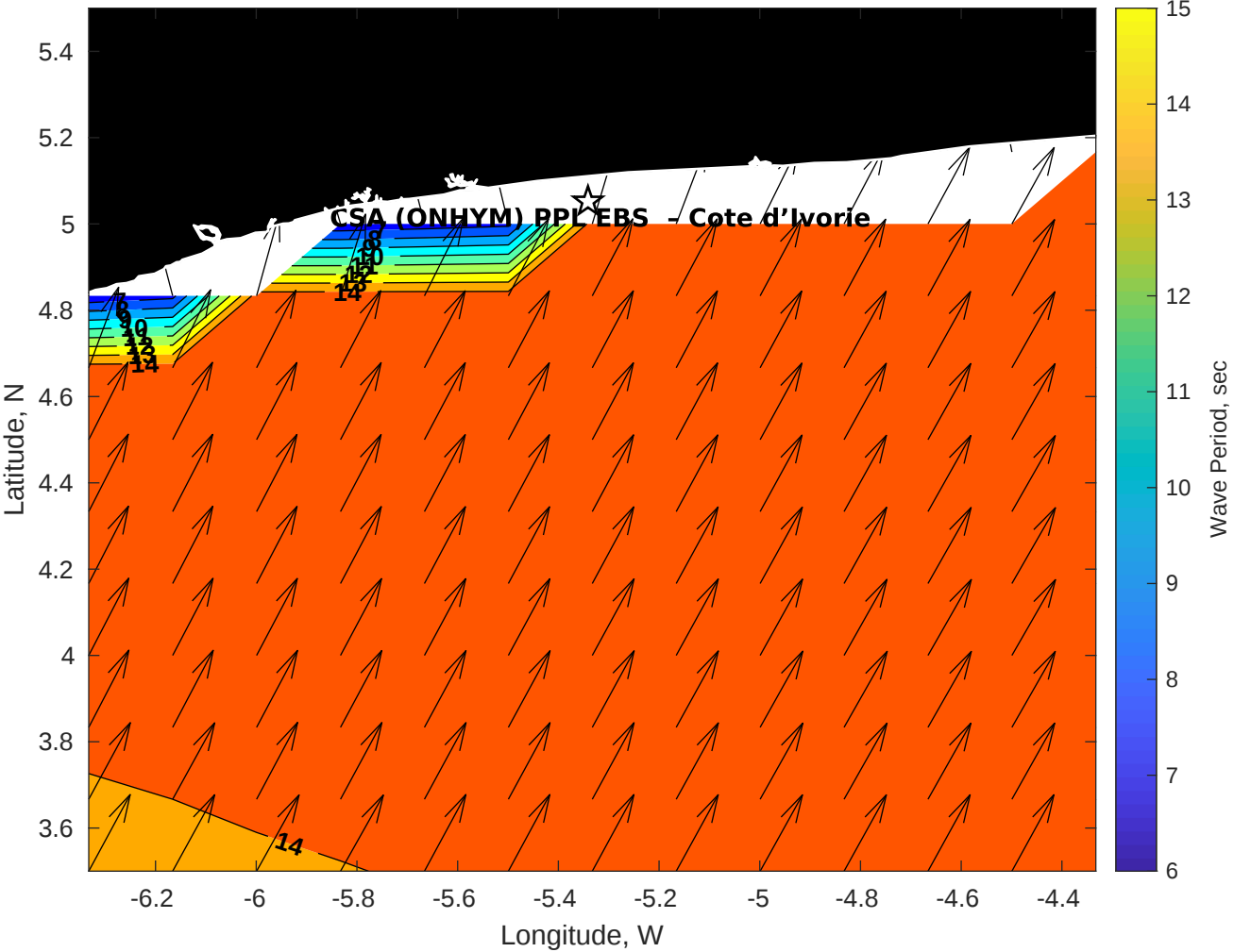
GFS Wave Period (sec) for CSA (ONHYM) PPL EBS - Cote d'Ivoire at 02-Dec-2025 09:00:00
