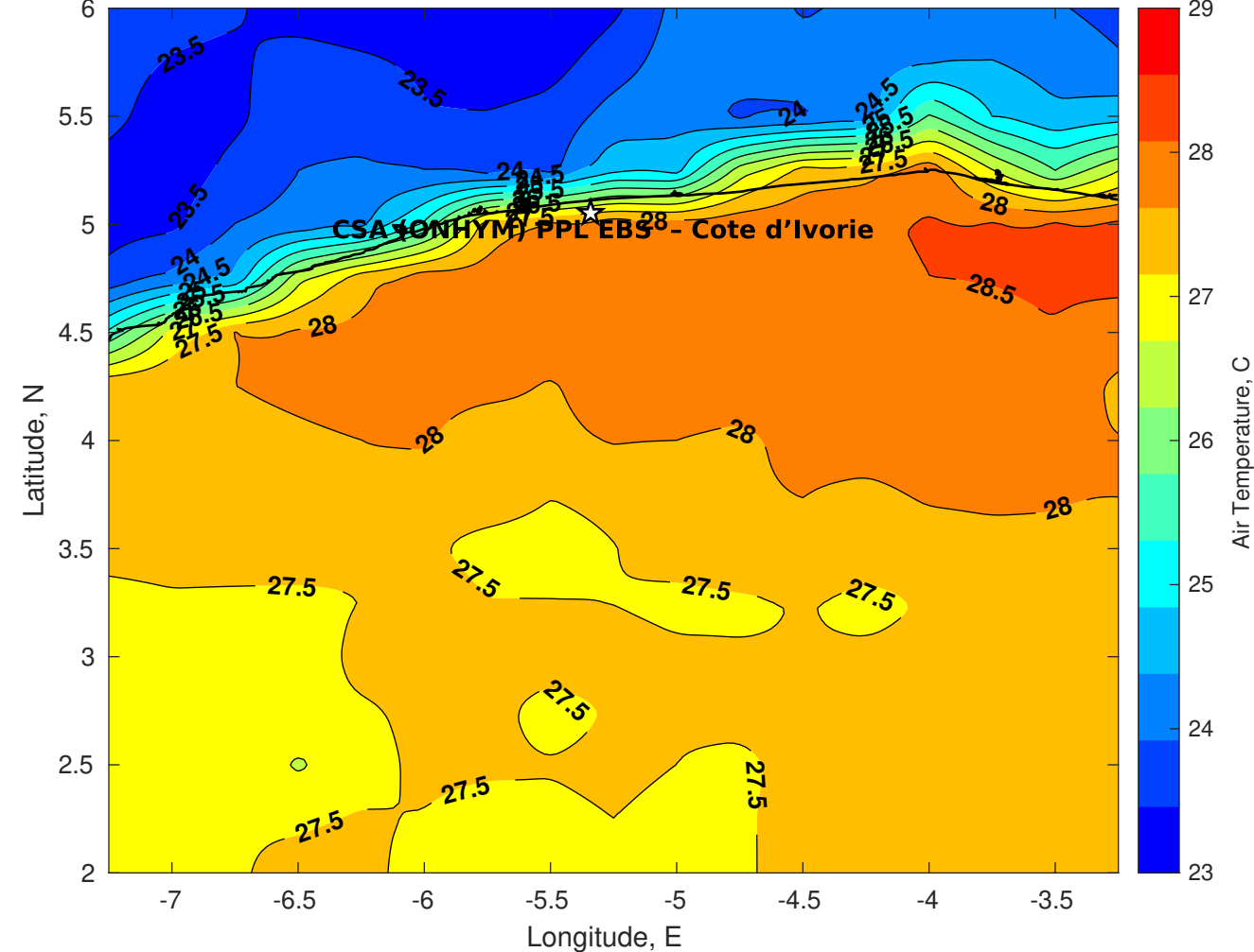
Air Temperature (C) for CSA (ONHYM) PPL EBS - Cote d'Ivoire at 02-Dec-2025
