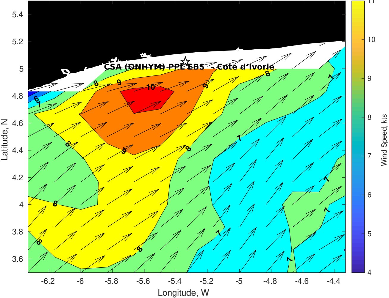
GFS Winds (kts) for CSA (ONHYM) PPL EBS - Cote d'Ivoire at 02-Dec-2025 09:00:00
