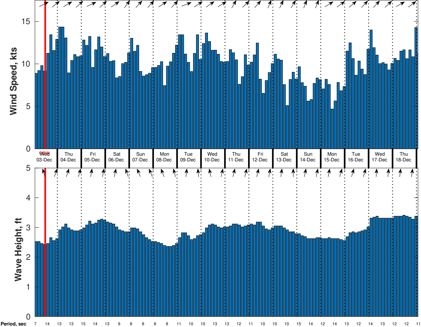
Wind & Wave Forecast for CSA (ONHYM) PPL EBS - Cote d'Ivoire from 02-Dec-2025 01:00:00 to 18-Dec-2025 01:00:00
