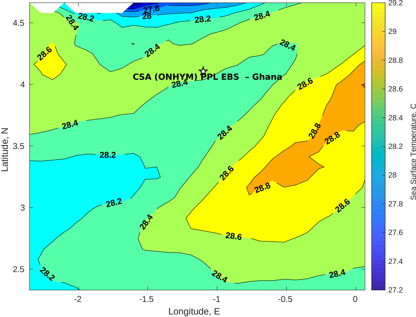
SST for CSA (ONHYM) PPL EBS - Ghana at 01-Dec-2025 00:00:00
