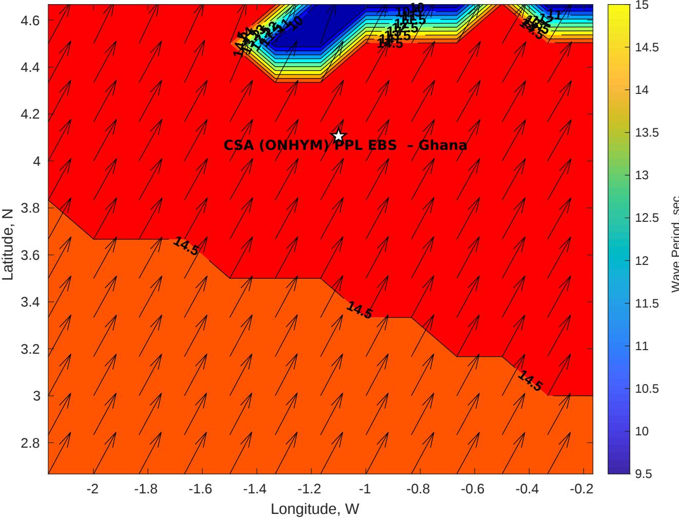
GFS Wave Period (sec) for CSA (ONHYM) PPL EBS - Ghana at 02-Dec-2025 09:00:00
