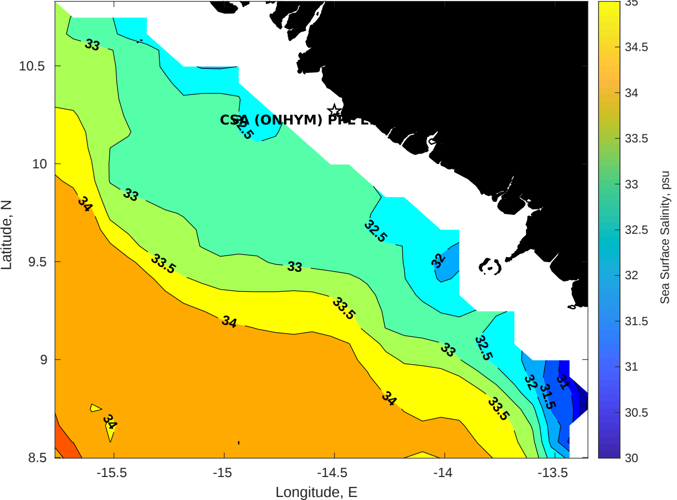
Surface Salinity for CSA (ONHYM) PPL EBS - Guinea at 01-Dec-2025 00:00:00
