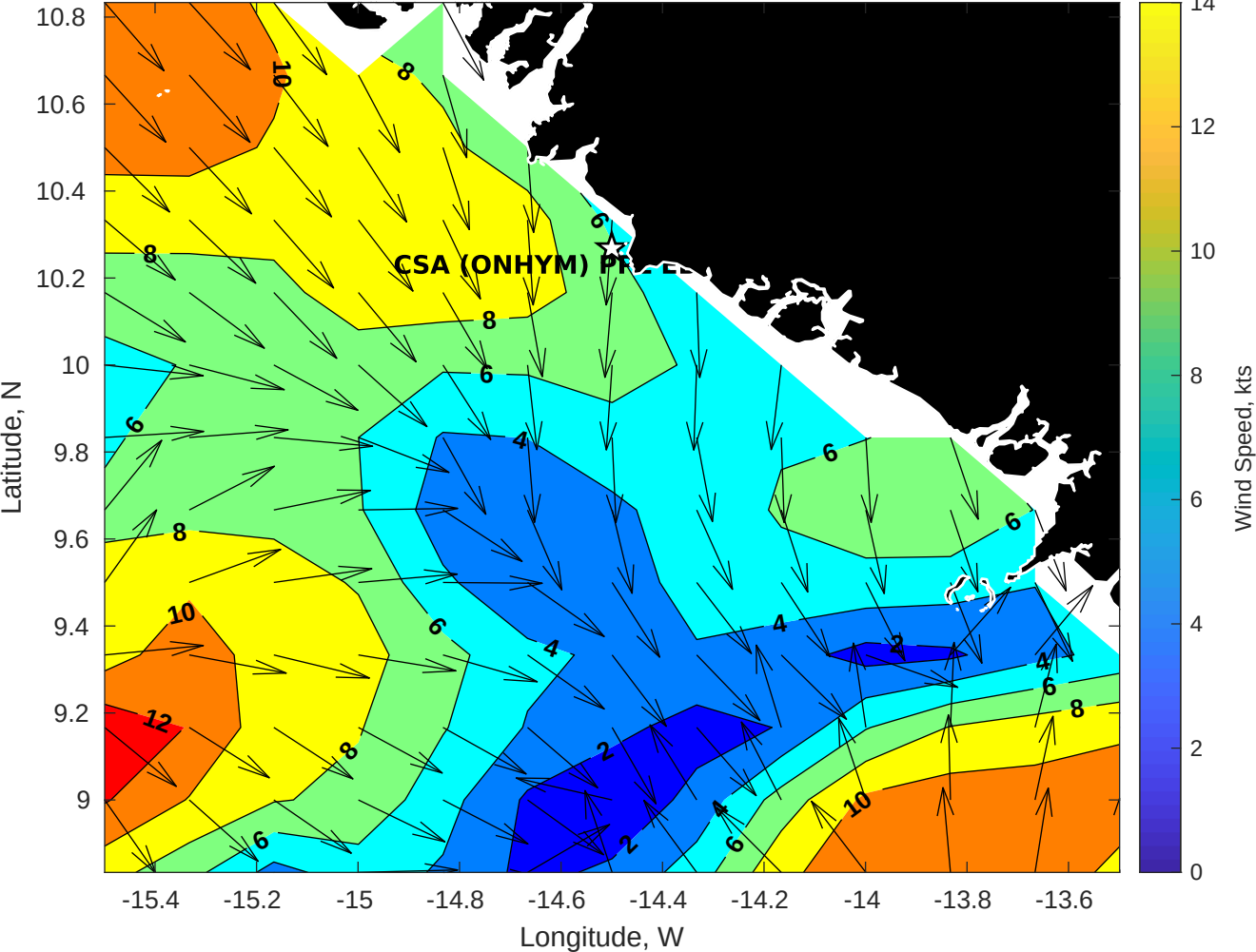
GFS Winds (kts) for CSA (ONHYM) PPL EBS - Guinea at 02-Dec-2025 09:00:00
