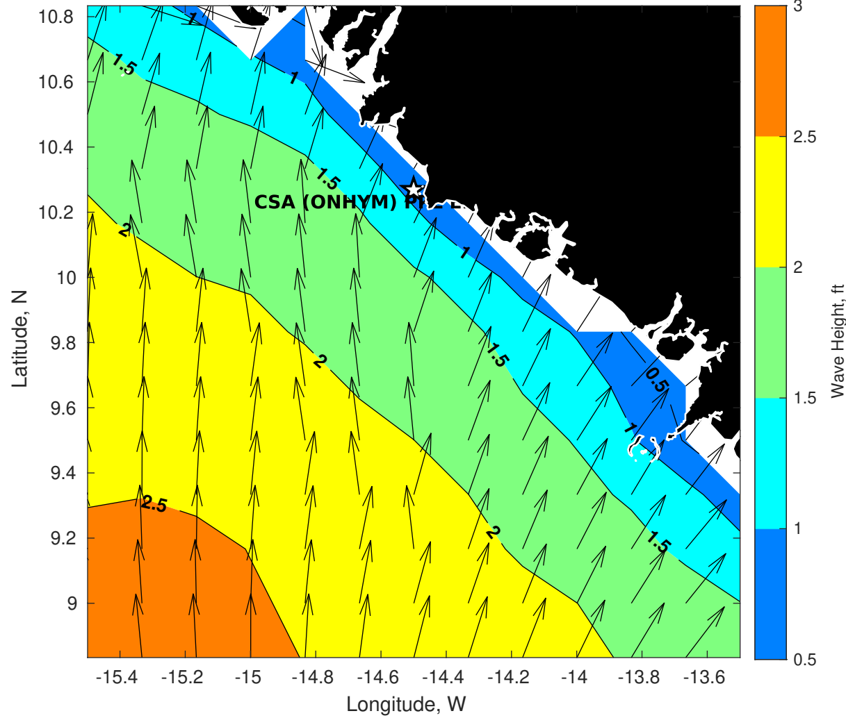
GFS Wave Height (ft) for CSA (ONHYM) PPL EBS - Guinea at 02-Dec-2025 09:00:00
