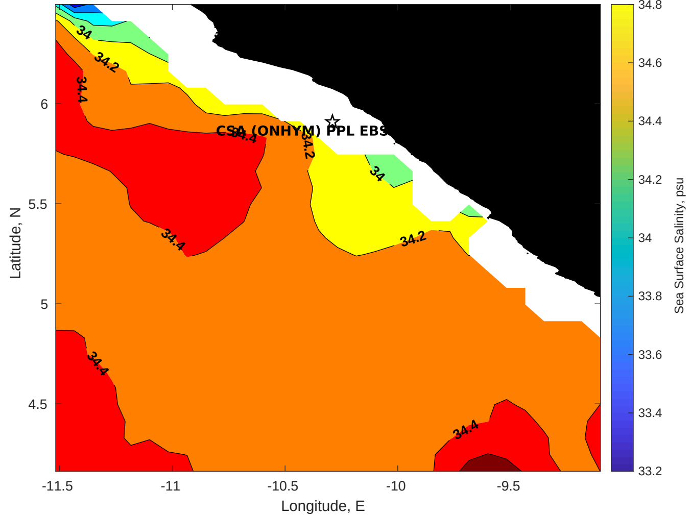
Surface Salinity for CSA (ONHYM) PPL EBS - Liberia at 01-Dec-2025 00:00:00
