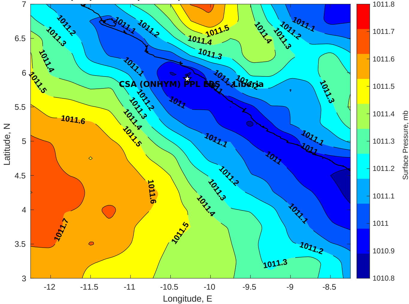
Surface Pressure (mb) for CSA (ONHYM) PPL EBS - Liberia at 03-Dec-2025 00:00:00
