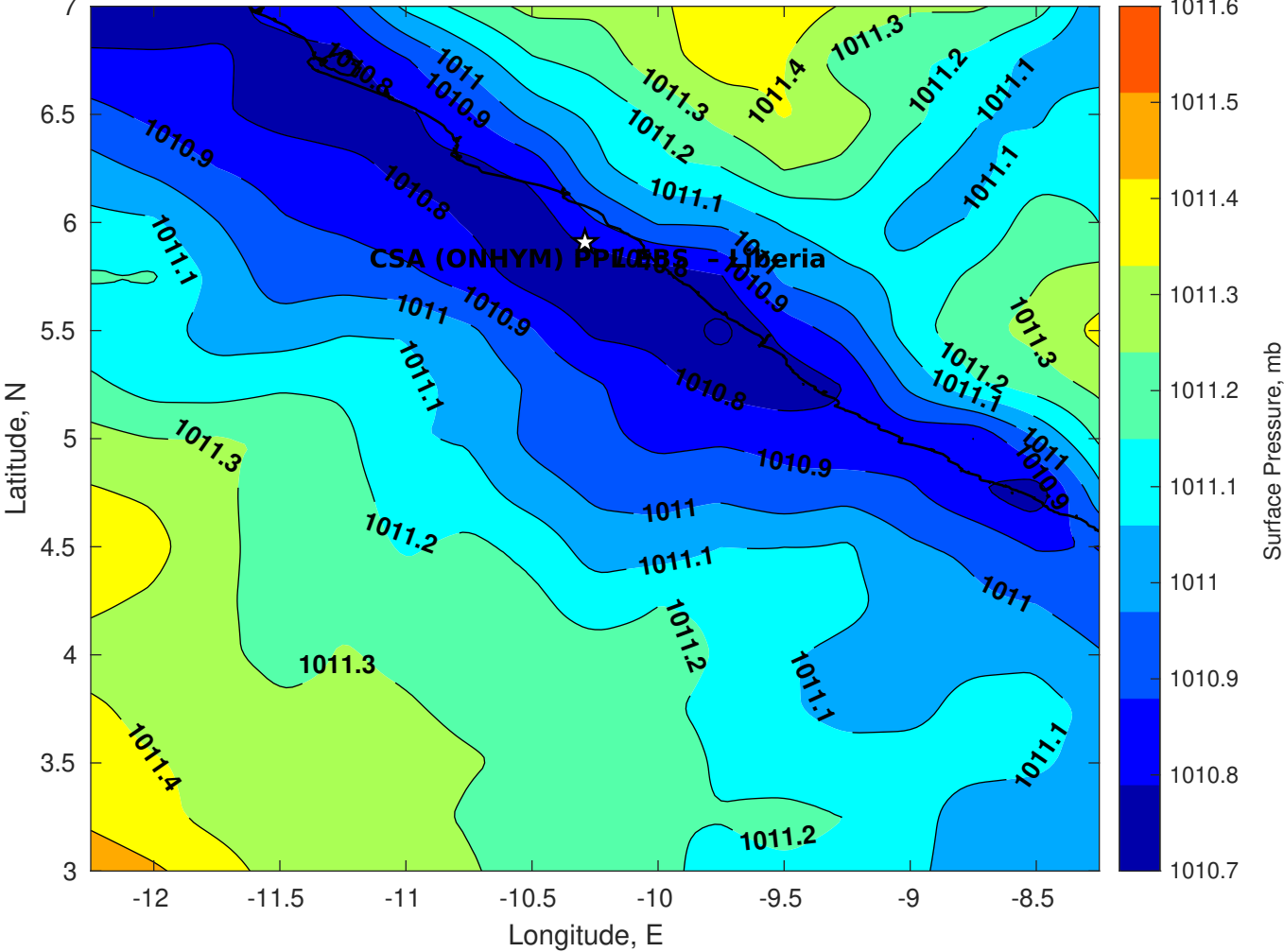
Surface Pressure (mb) for CSA (ONHYM) PPL EBS - Liberia at 04-Dec-2025 00:00:00
