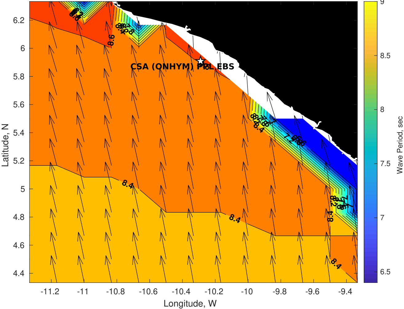
GFS Wave Period (sec) for CSA (ONHYM) PPL EBS - Liberia at 02-Dec-2025 09:00:00
