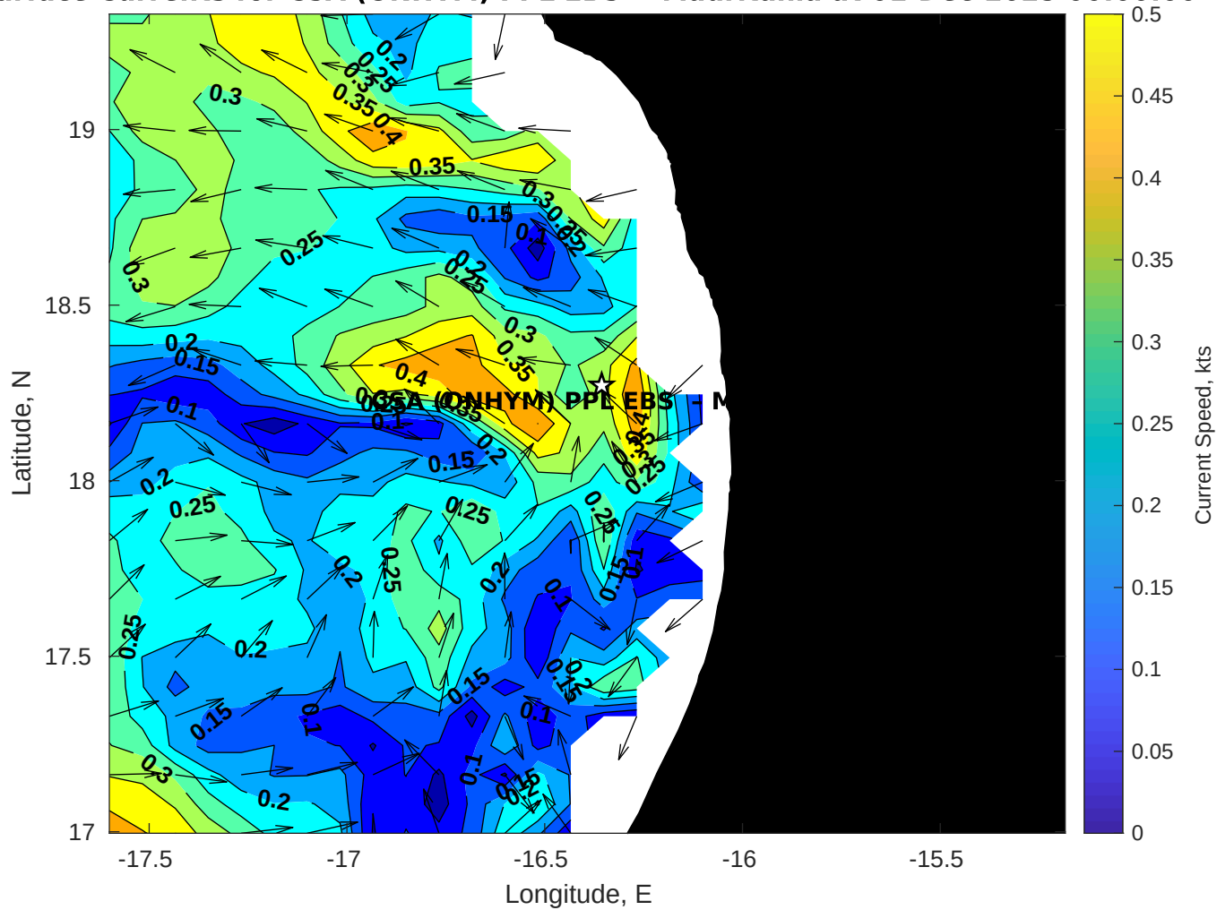
Surface Currents for CSA (ONHYM) PPL EBS - Mauritania at 01-Dec-2025 00:00:00
