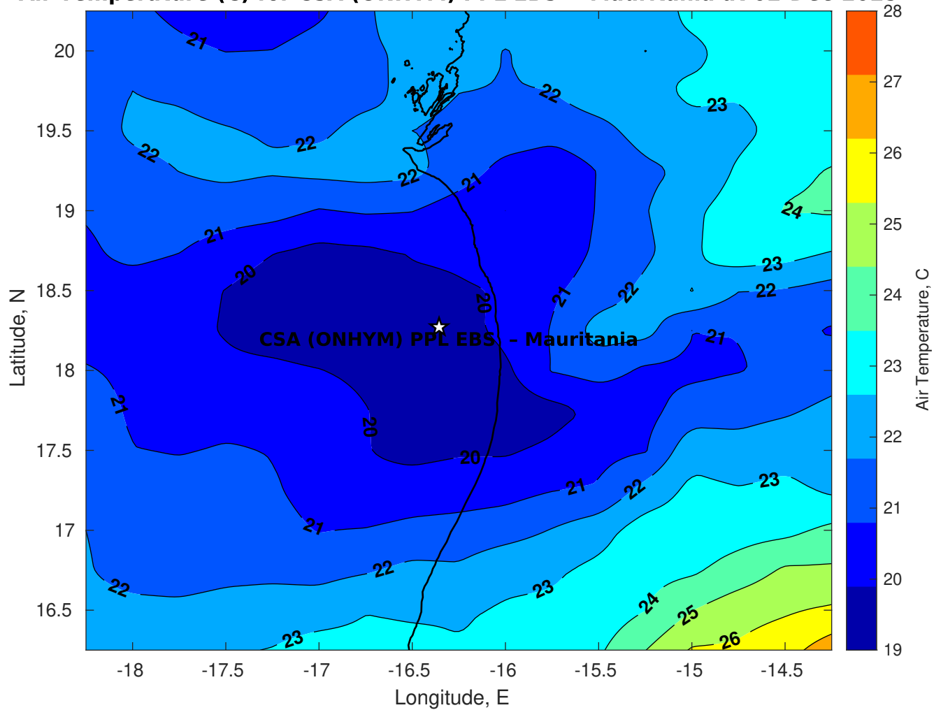
Air Temperature (C) for CSA (ONHYM) PPL EBS - Mauritania at 02-Dec-2025
