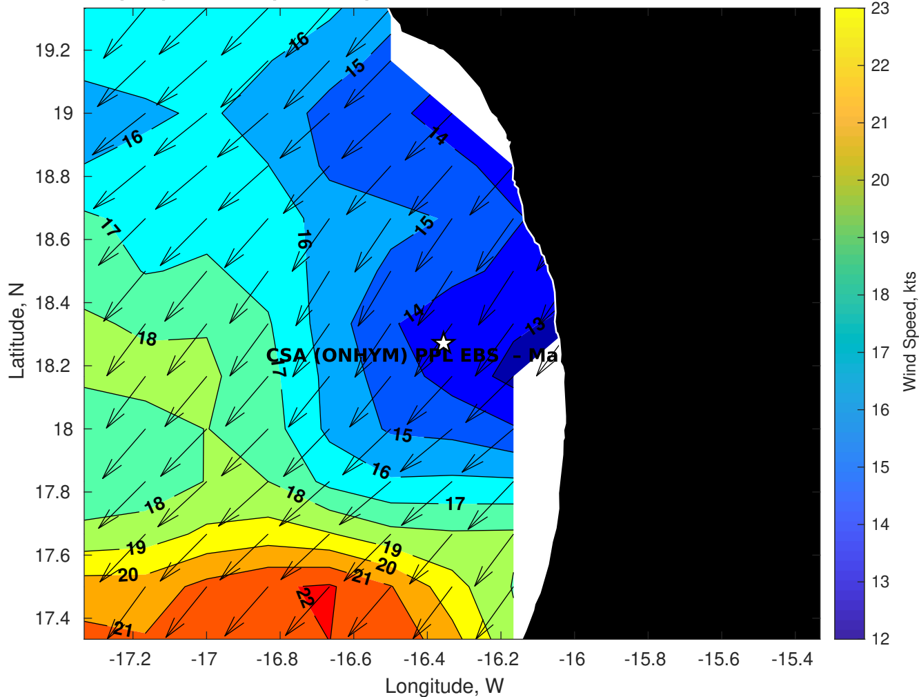
GFS Winds (kts) for CSA (ONHYM) PPL EBS - Mauritania at 02-Dec-2025 09:00:00
