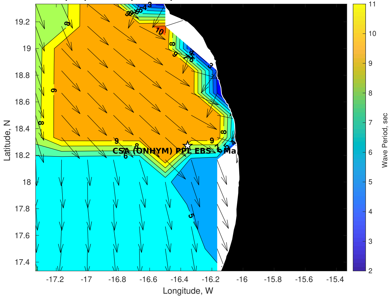
GFS Wave Period (sec) for CSA (ONHYM) PPL EBS - Mauritania at 02-Dec-2025 09:00:00
