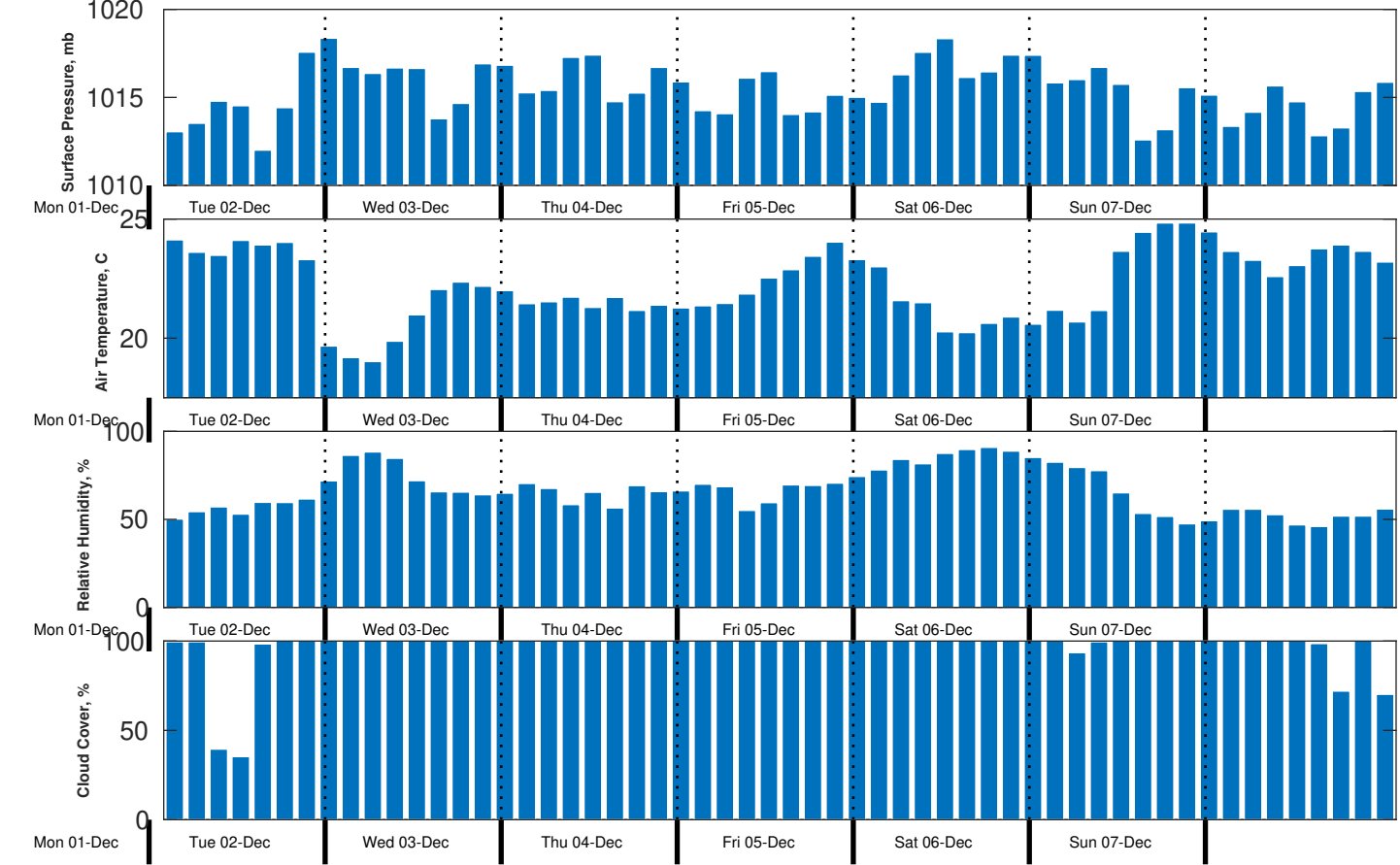
Met Forecast for CSA (ONHYM) PPL EBS - Mauritania from 02-Dec-2025 00:00:00 to 09-Dec-2025 00:00:00
