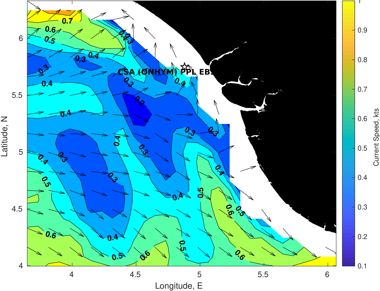
Surface Currents for CSA (ONHYM) PPL EBS - Nigeria at 01-Dec-2025 00:00:00
