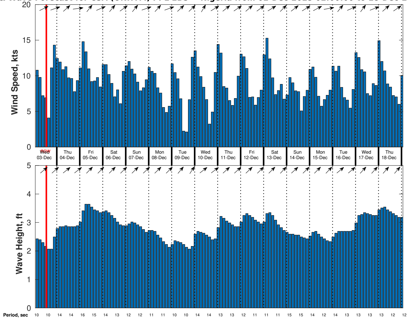
Wind & Wave Forecast for CSA (ONHYM) PPL EBS - Nigeria from 02-Dec-2025 02:00:00 to 18-Dec-2025 02:00:00
