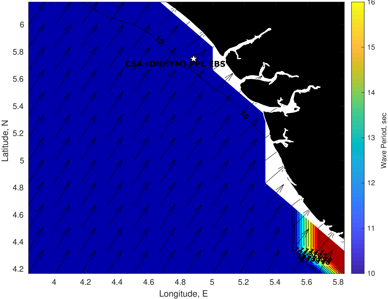
GFS Wave Period (sec) for CSA (ONHYM) PPL EBS - Nigeria at 02-Dec-2025 09:00:00
