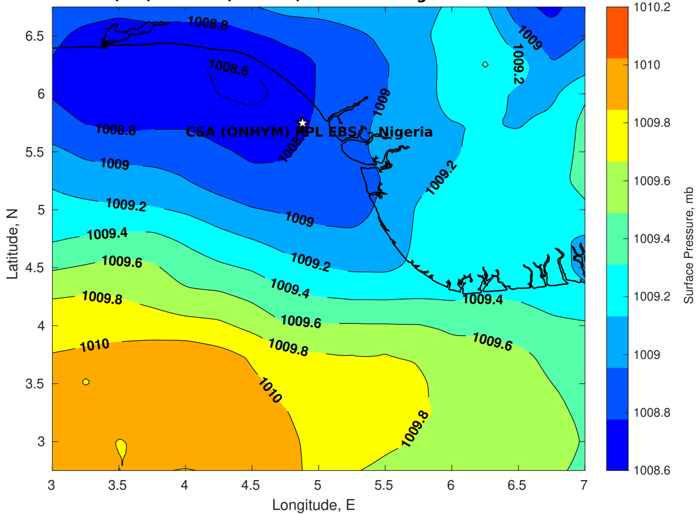
Surface Pressure (mb) for CSA (ONHYM) PPL EBS - Nigeria at 04-Dec-2025 00:00:00
