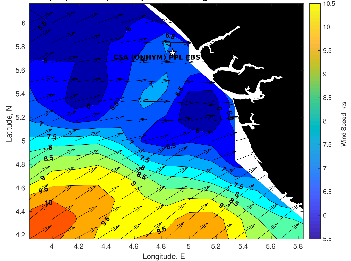
GFS Winds (kts) for CSA (ONHYM) PPL EBS - Nigeria at 02-Dec-2025 09:00:00
