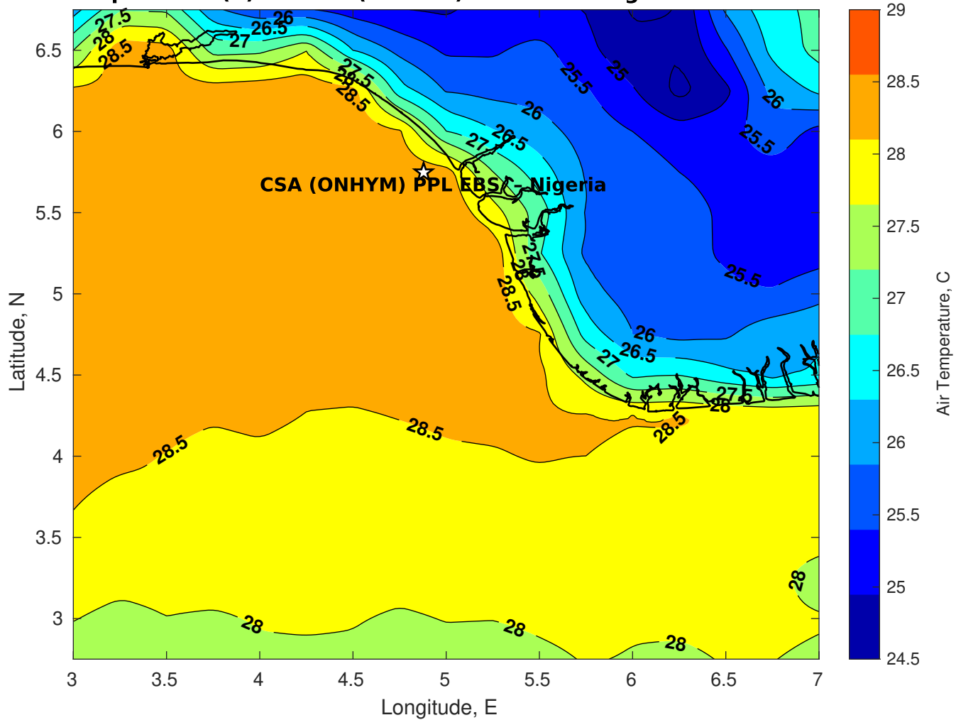
Air Temperature (C) for CSA (ONHYM) PPL EBS - Nigeria at 02-Dec-2025
