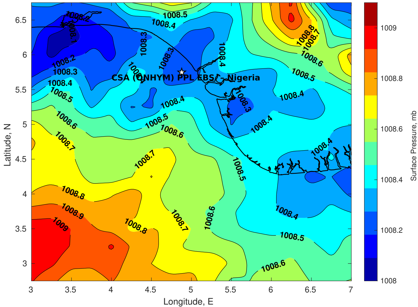
Surface Pressure (mb) for CSA (ONHYM) PPL EBS - Nigeria at 02-Dec-2025 00:00:00
