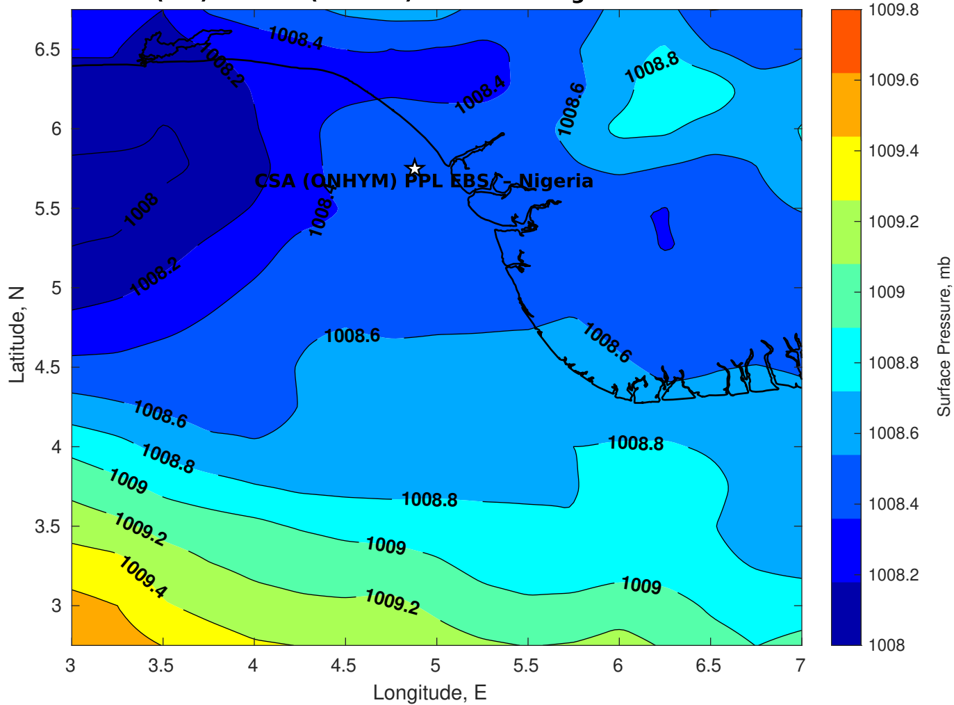
Surface Pressure (mb) for CSA (ONHYM) PPL EBS - Nigeria at 03-Dec-2025 00:00:00
