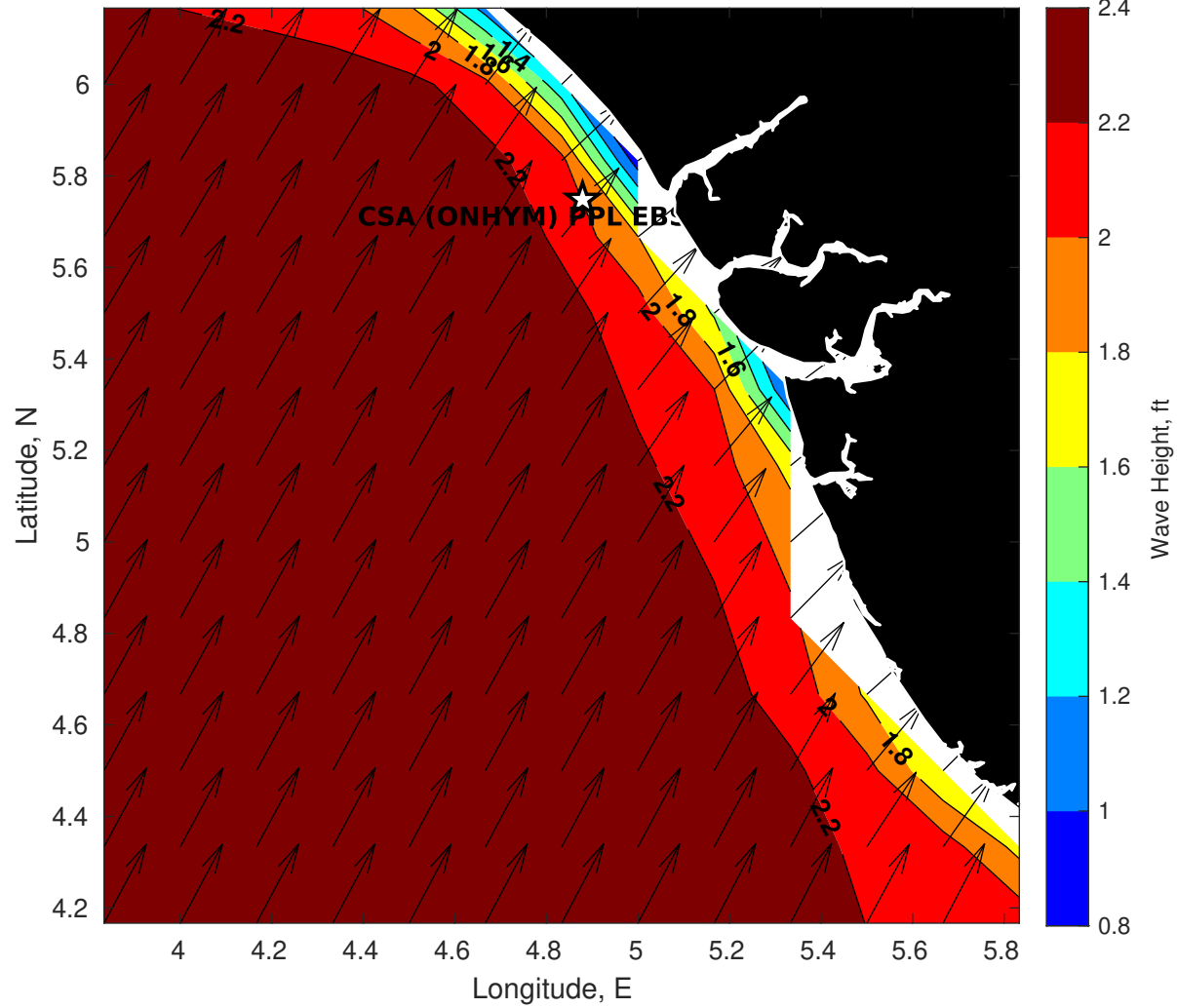
GFS Wave Height (ft) for CSA (ONHYM) PPL EBS - Nigeria at 02-Dec-2025 09:00:00
