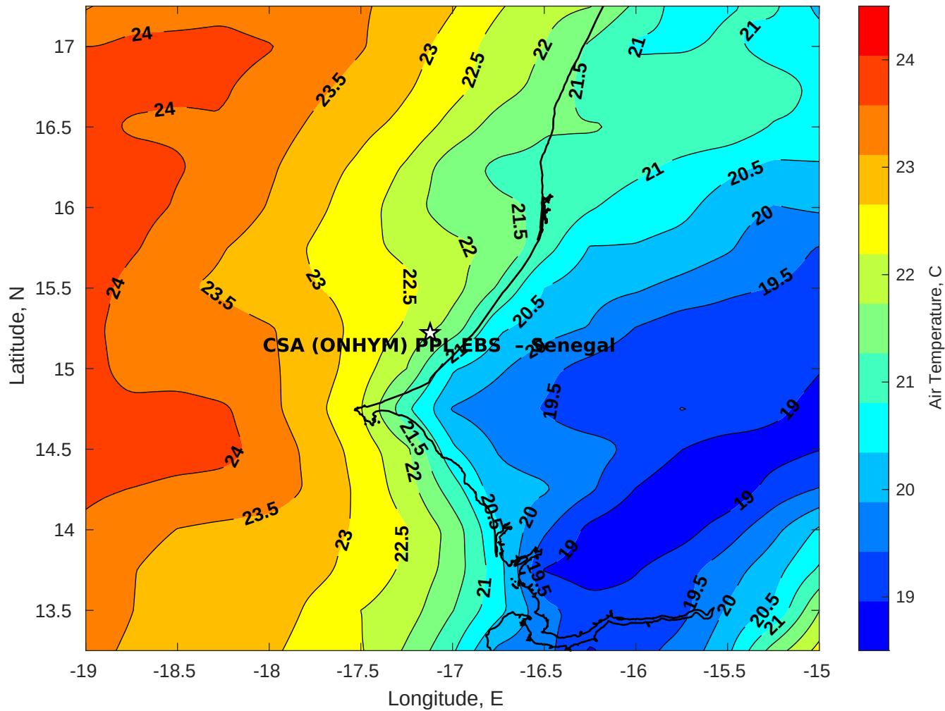
Air Temperature (C) for CSA (ONHYM) PPL EBS - Senegal at 02-Dec-2025
