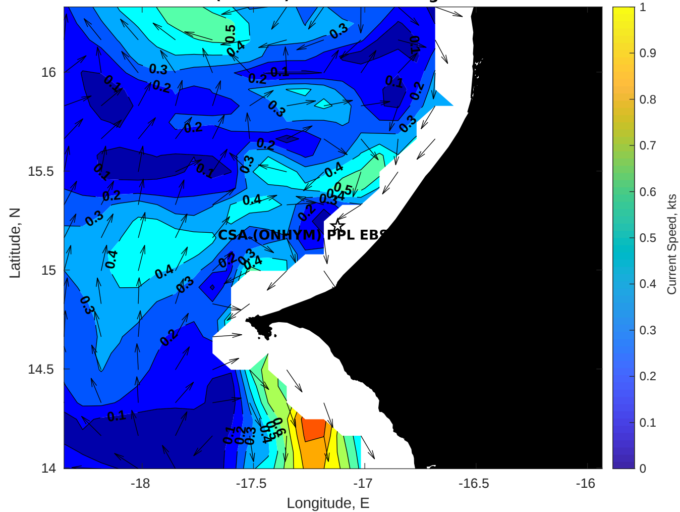
Surface Currents for CSA (ONHYM) PPL EBS - Senegal at 01-Dec-2025 00:00:00
