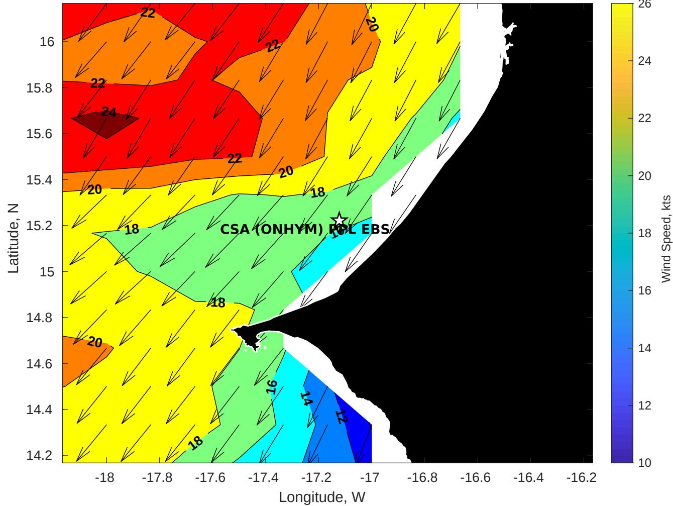
GFS Winds (kts) for CSA (ONHYM) PPL EBS - Senegal at 02-Dec-2025 09:00:00
