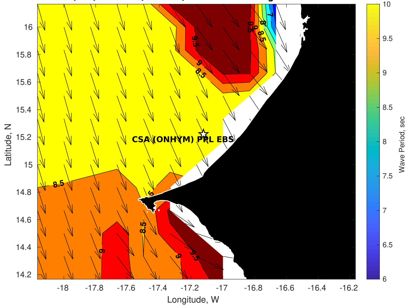
GFS Wave Period (sec) for CSA (ONHYM) PPL EBS - Senegal at 02-Dec-2025 09:00:00
