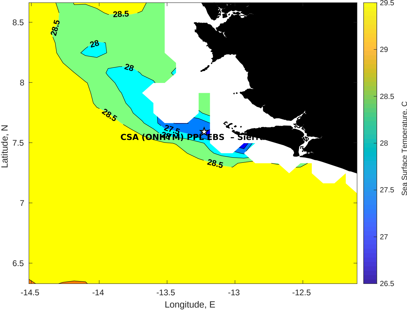
SST for CSA (ONHYM) PPL EBS - Sierra Leone at 01-Dec-2025 00:00:00
