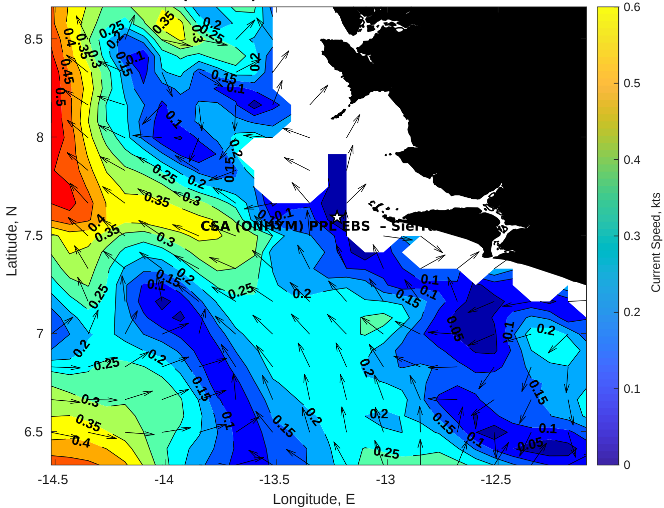
Surface Currents for CSA (ONHYM) PPL EBS - Sierra Leone at 01-Dec-2025 00:00:00
