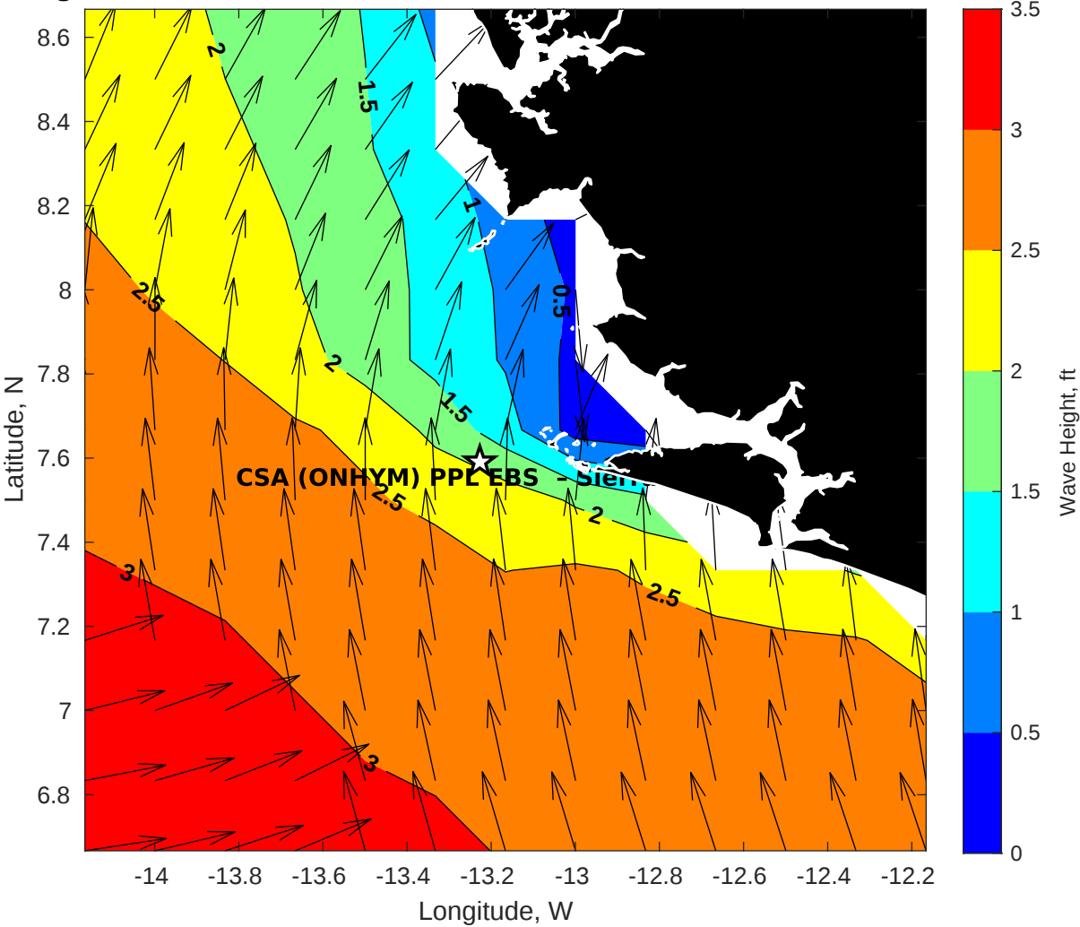
GFS Wave Height (ft) for CSA (ONHYM) PPL EBS - Sierra Leone at 02-Dec-2025 09:00:00
