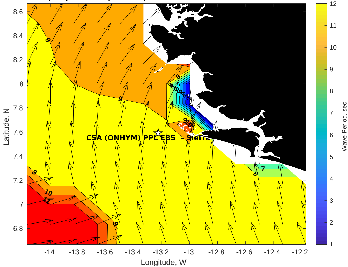
GFS Wave Period (sec) for CSA (ONHYM) PPL EBS - Sierra Leone at 02-Dec-2025 09:00:00
