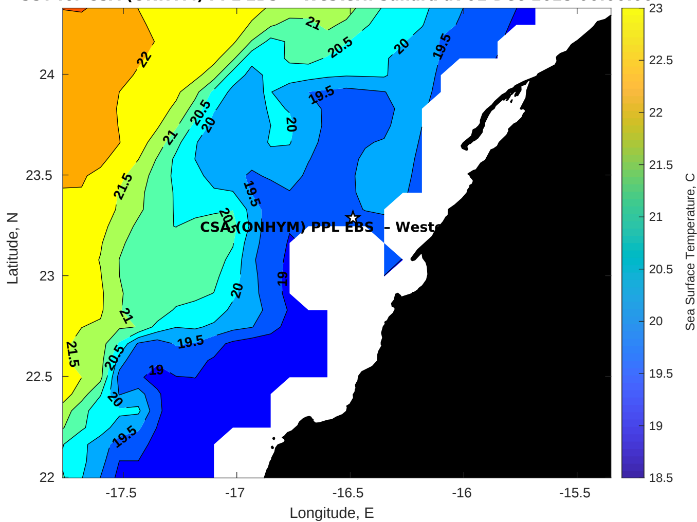
SST for CSA (ONHYM) PPL EBS - Western Sahara at 01-Dec-2025 00:00:00
