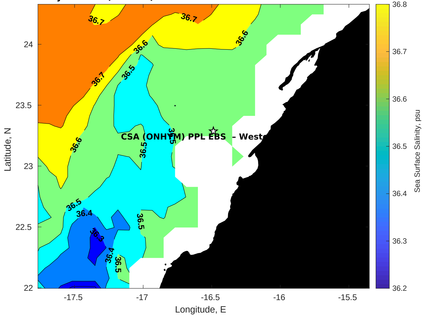
Surface Salinity for CSA (ONHYM) PPL EBS - Western Sahara at 01-Dec-2025 00:00:00
