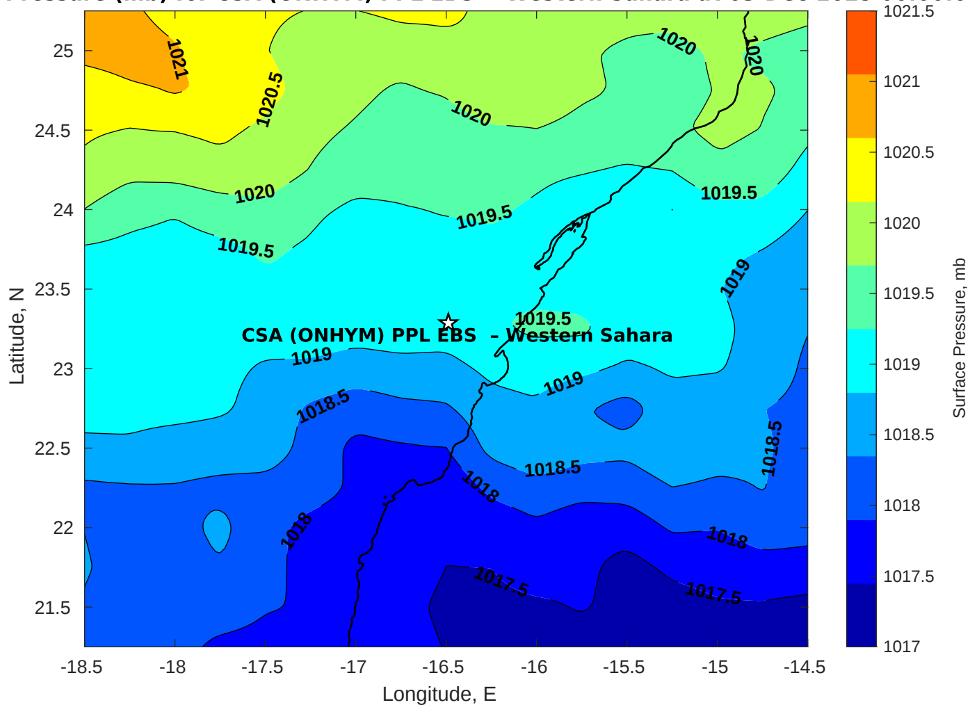
Surface Pressure (mb) for CSA (ONHYM) PPL EBS - Western Sahara at 03-Dec-2025 00:00:00
