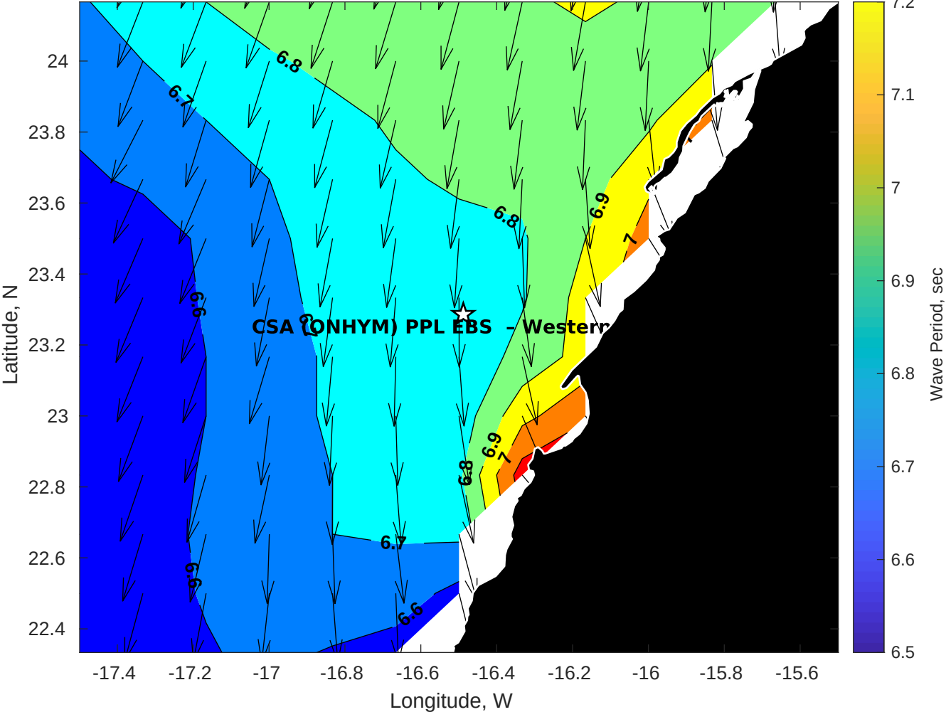
GFS Wave Period (sec) for CSA (ONHYM) PPL EBS - Western Sahara at 02-Dec-2025 09:00:00
