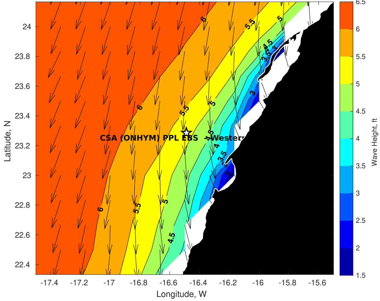
GFS Wave Height (ft) for CSA (ONHYM) PPL EBS - Western Sahara at 02-Dec-2025 09:00:00
