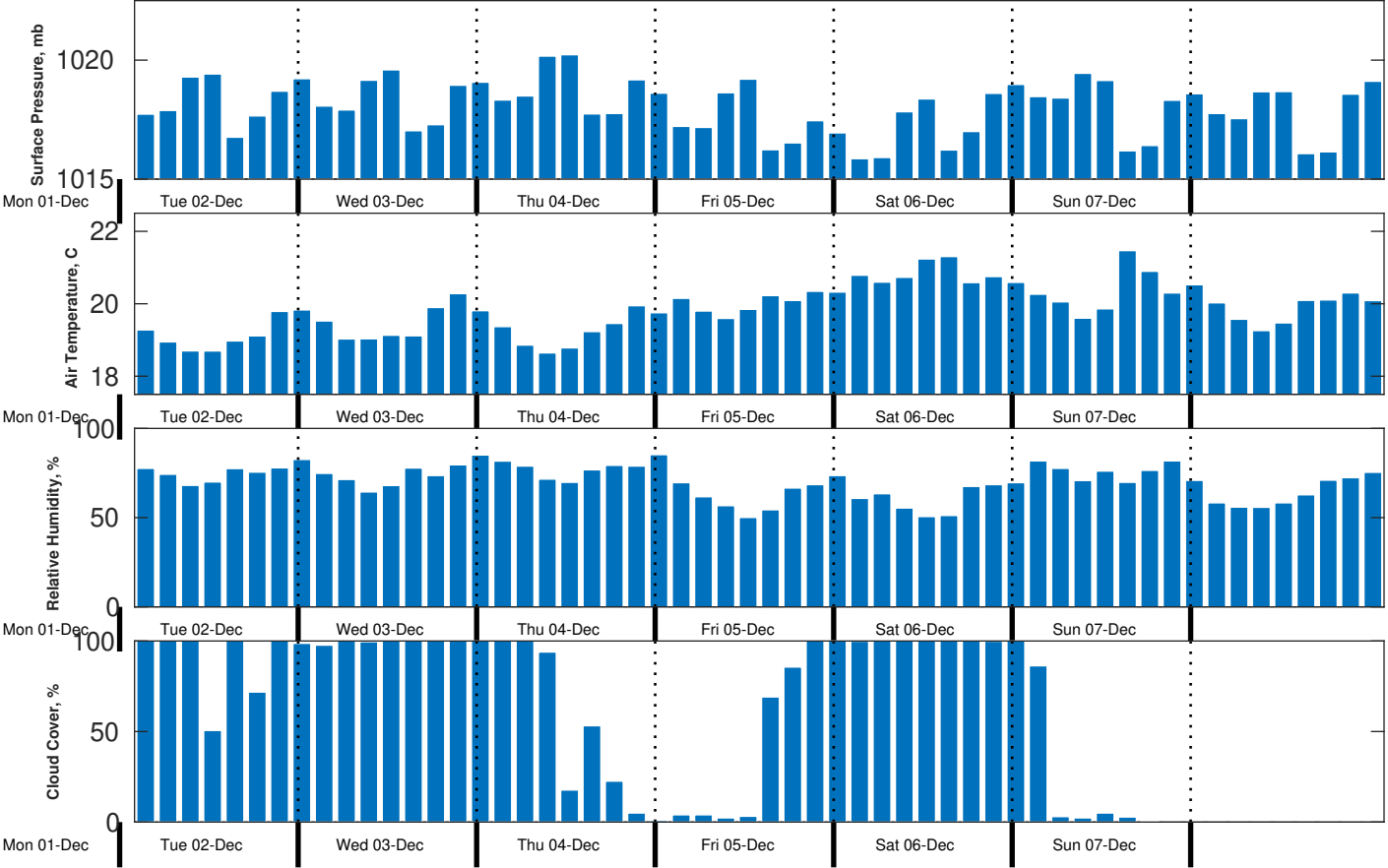
Met Forecast for CSA (ONHYM) PPL EBS - Western Sahara from 02-Dec-2025 00:00:00 to 09-Dec-2025 00:00:00
