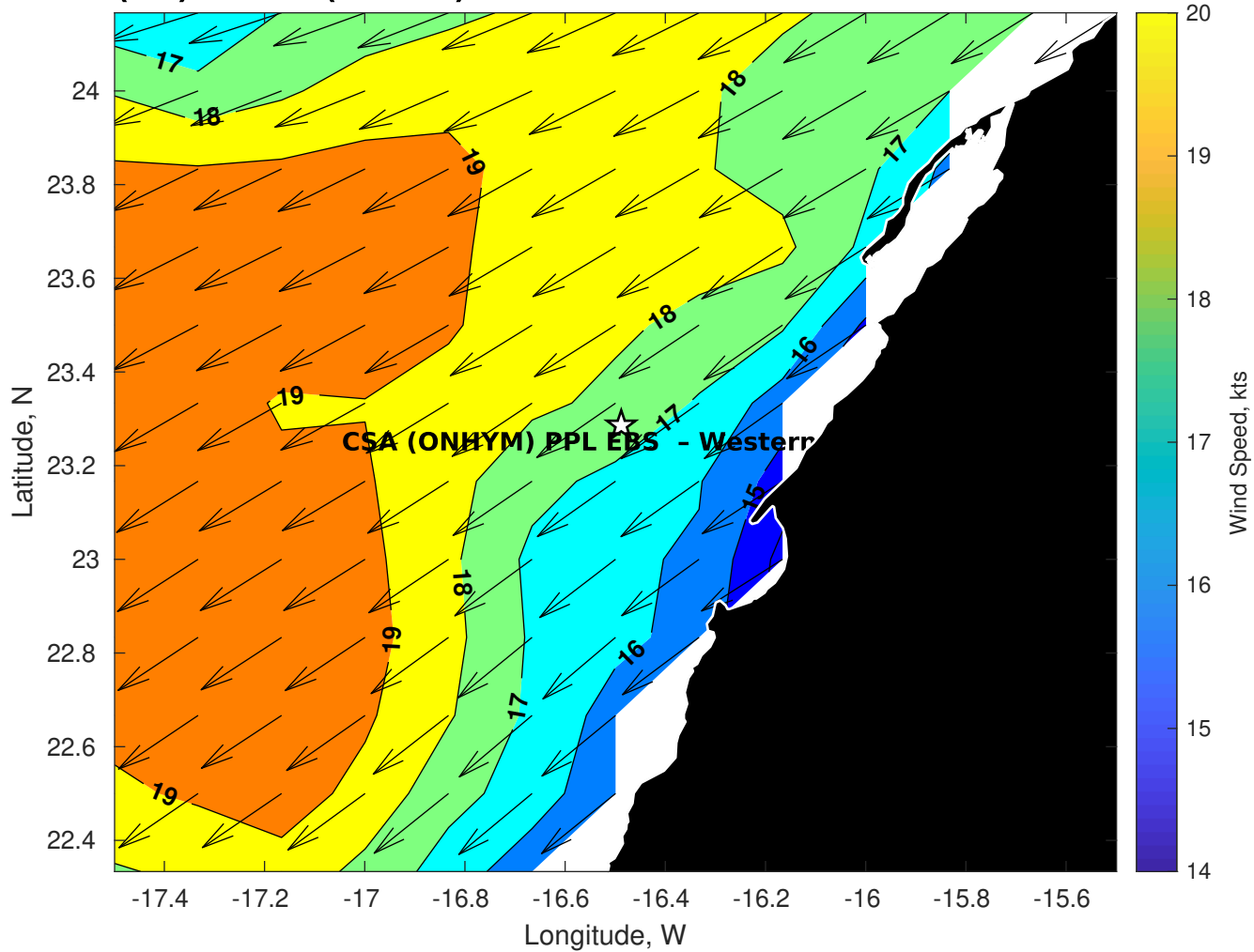
GFS Winds (kts) for CSA (ONHYM) PPL EBS - Western Sahara at 02-Dec-2025 09:00:00
