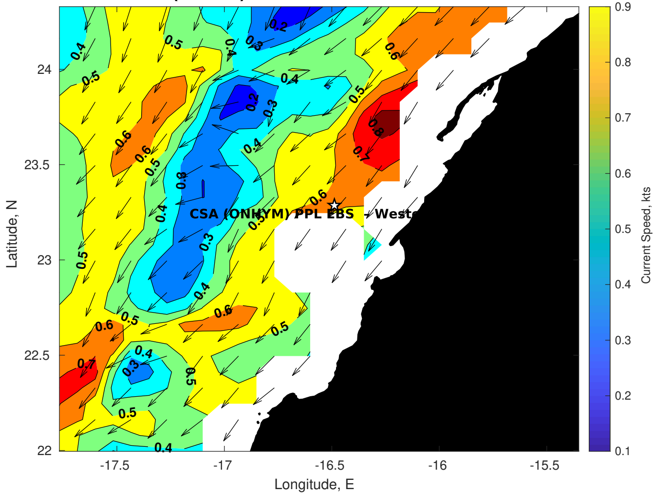
Surface Currents for CSA (ONHYM) PPL EBS - Western Sahara at 01-Dec-2025 00:00:00
