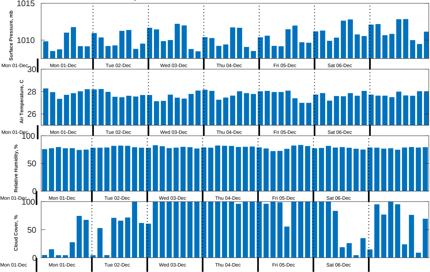
Met Forecast for Gyre from 01-Dec-2025 20:00:00 to 08-Dec-2025 20:00:00
